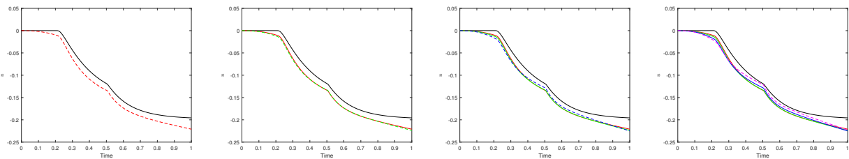
Figure 9. Response to a multiple stimuli (two stimuli in sequence). Time evolution of the ionic variable u at midpoint of heart with \beta = 1 and \alpha = — 1, — 0.925, — 0.9, — 0.85, — 0.8.
