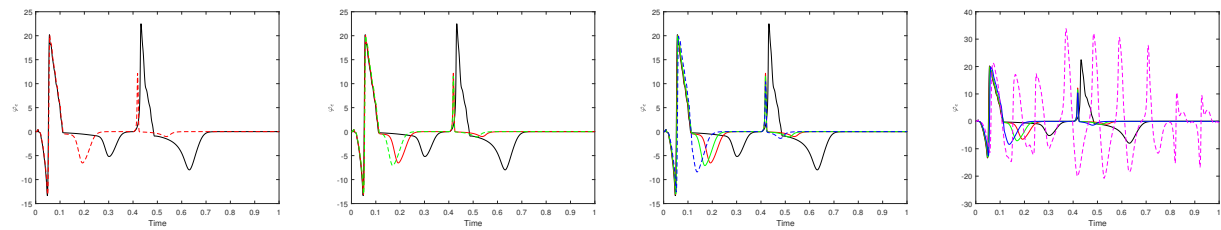
Figure 23. Response to a multiple stimuli (two stimuli in sequence). Time evolution of the extracellular potential \phi_e at midpoint of heart with \alpha = 1 and \beta = 1, 0.925, 0.9, 0.85, 0.8 .
