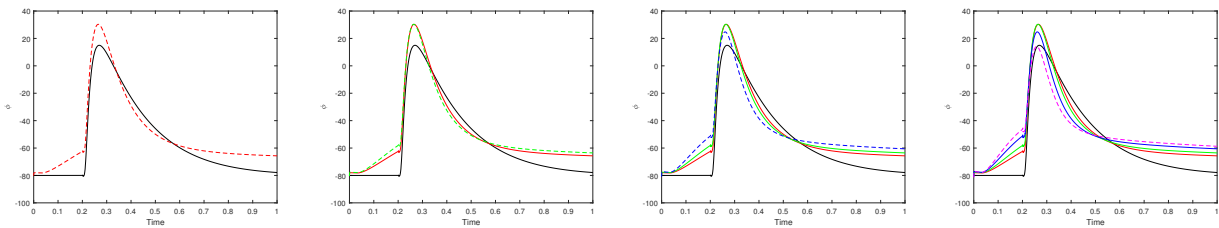
Figure 4. Response to a single stimulus. Time evolution of the transmembrane potential \phi at midpoint of heart with \beta = 1 and \alpha = \text{---} 1, \text{---} 0.925, \text{---} 0.9, \text{---} 0.85, \text{---} 0.8 .
