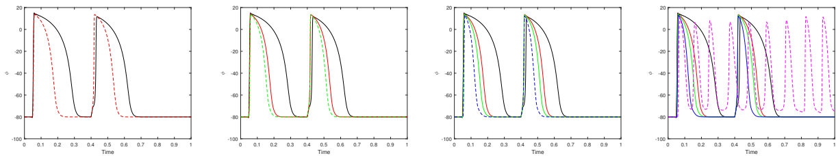
Figure 22. Response to a multiple stimuli (two stimuli in sequence). Time evolution of the transmembrane potential \phi at midpoint of heart with \alpha = 1 and \beta = 1, 0.925, 0.9, 0.85, 0.8 .
