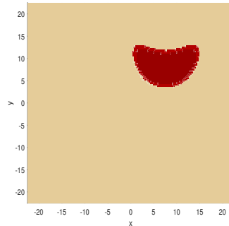
Figure 3. Heart-torso domain.
