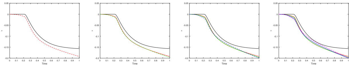
Figure 6. Response to a single stimulus. Time evolution of the ionic variable u at midpoint of heart \beta = 1 and \alpha = \text{---} 1, \text{---} 0.925, \text{---} 0.9, \text{---} 0.85, \text{---} 0.8 .
