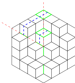
Figure 4: Running example in the proof of Proposition 2.1.
