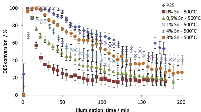
Fig. 12. Diethylsulfide conversion under UV-A illumination on Sn-doped TiO 2 calcined at 500 °C, influence of Sn content.
