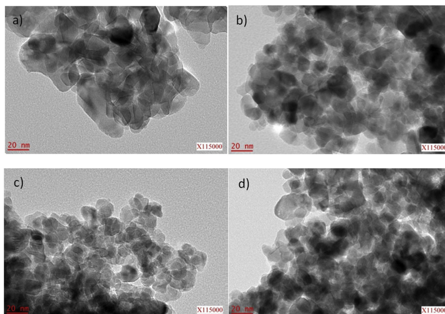
Fig. 5. TEM images of undoped and Sn-doped nanoparticles calcined at 380 °C: a) TiO 2 , b) 1%Sn-TiO 2 , c) 4%Sn-TiO 2 , d) 8%Sn-TiO 2 .
