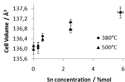
Fig. 3. Cell volume of TiO 2 anatase calculated with the cell parameters obtained from profile matching of undoped and Sn-doped nanoparticles calcined at 380 °C and 500 °C.
