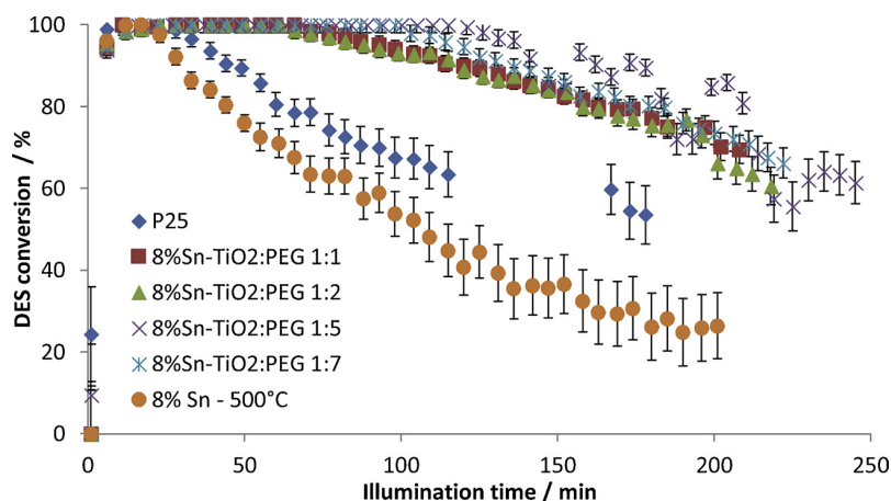
Fig. 13. Diethyl sulfide conversion under UV-A illumination on 8%Sn-TiO 2 samples calcined at 500 °C : influence of PEG content.
