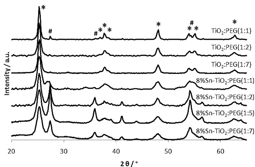
Fig. 4. XRD pattern of undoped and Sn-doped nanoparticles synthesized with PEG calcined at 500 °C, *: anatase, #: rutile.
