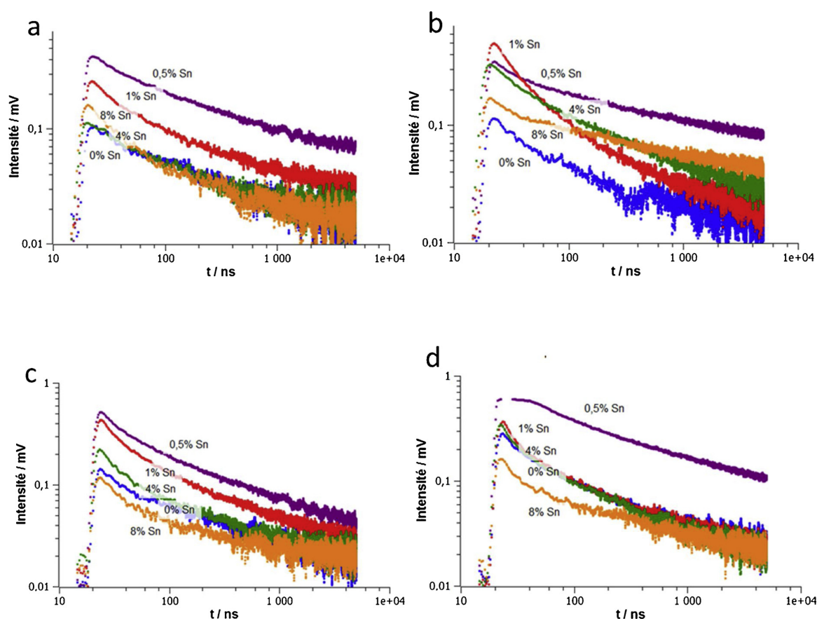
Fig. 10. TRMC signal obtained by irradiation of Sn-doped TiO 2 a) calcined at 380 °C and excited at 355 nm, b) calcined at 500 °C and excited at 355 nm, c) calcined at 380 °C and excited at 450 nm, d) calcined at 500 °C and excited at 450 nm.
