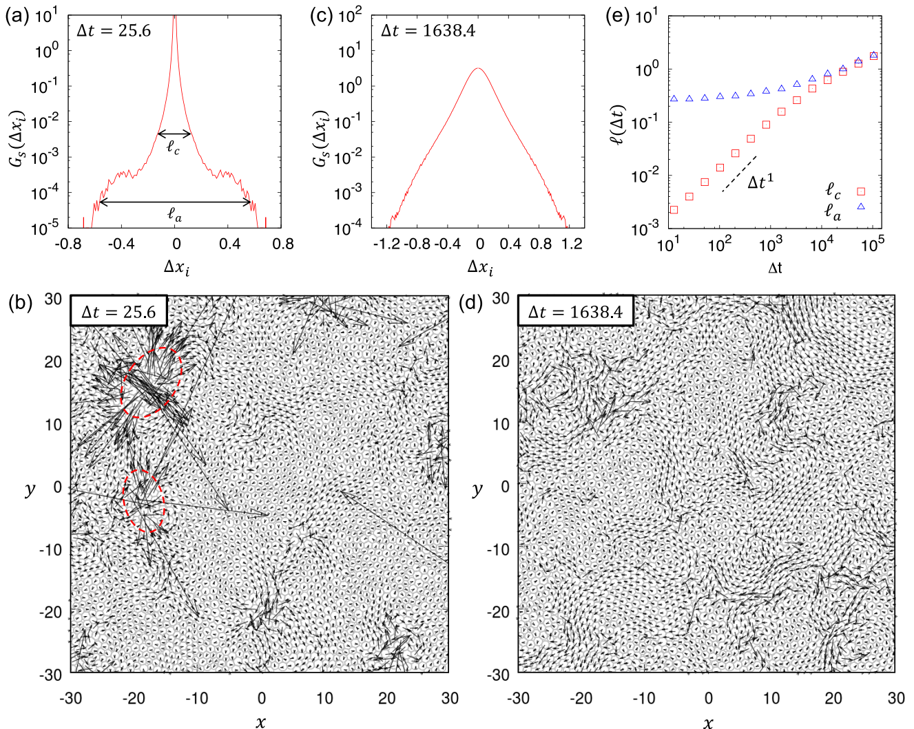
FIG. 4. (a,c) Van Hove particle distribution, Eq. (13), for t_w = 104\,858.0 . In (a) there is a clear separation of lengthscales into \ell_a and \ell_c . (b,d) Nonaffine displacement fields \Delta \mathbf{r}_i corresponding to (a,c); the field is magnified by a factor of 120 and 4, respectively, for better visibility. Division events are highlighted with dashed circles in (b). (e) Time evolution of the lengthscales \ell_a and \ell_c .
