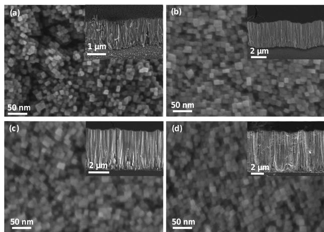
Figure 6. Top- and side-view SEM images (in inset) of rutile \text{TiO}_2 NR films grown at 150^\circ\text{C} for 8 h with different volumes of TTIP in a mixture (1:1) of hydrochloric acid and ethanol: (a) 0.25 mL, (b) 1 mL, (c) 2 mL, and (d) 3 mL.
