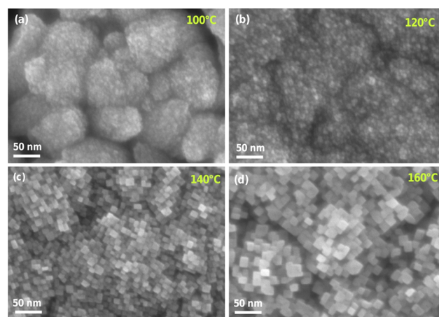
Figure 2. Top-surface SEM images of rutile TiO 2 films grown at different synthesis temperatures: (a) 100 °C, (b) 120 °C, (c) 140 °C, and (d) 160 °C (keeping the other parameters constant).
