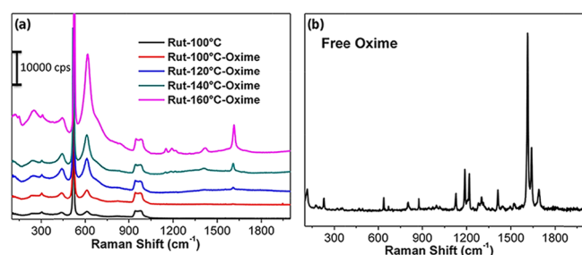
Figure 3. (a) Raman spectra of rutile nanorods synthesized at different growth temperatures and functionalized with oxime. (b) Raman spectra of free oxime molecules used for anchoring on each rutile \text{TiO}_2 nanorod surface.
