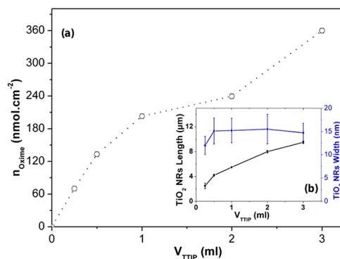
Figure 7. (a) Oxime loading onto \text{TiO}_2 nanorods synthesized at different TTIP volumes. (b) Influence of the TTIP volume on the length and the diameter of the nanorods.
