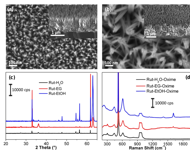
Figure 5. Top and cross-sectional (inset) SEM images of rutile TiO 2 NRs prepared by replacing ethanol with (a) ethylene glycol and (b) water in the presence of hydrochloric acid and 0.25 mL of TTIP at 150 °C for 8 h. (c) XRD of the nanostructure prepared with water, ethylene glycol, and ethanol. (d) Raman spectra of the three different nanostructures functionalized with oxime molecules.
