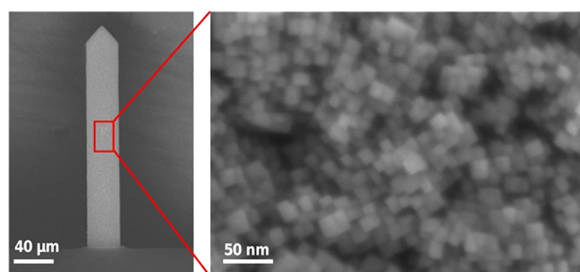
Figure 8. TiO 2 nanostructured cantilever prepared in ethanol, hydrochloric acid, 0.5 mL of TEACl, and 0.5 mL of TTIP at 150 °C for 8 h.
