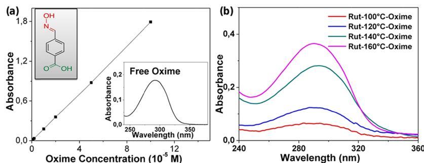
Figure 4. (a) UV–vis oxime calibration curve and UV–vis absorption spectrum of the free oxime molecule in NaOH solution (pH 12). Inset shows the scheme of the oxime molecule (the green part is the tethering site for the \text{TiO}_2 nanostructure, and the red one is the oxime function). (b) UV–vis spectra of desorbed oxime anchored on each rutile \text{TiO}_2 nanorod surface.
