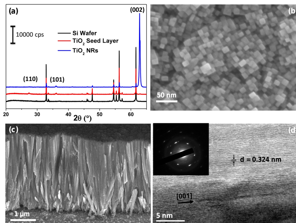
Figure 1. (a) XRD patterns of the as-prepared TiO 2 NR film (blue), TiO 2 seed layer made by sputtering (red), and a silicon wafer substrate as a reference (black). (b, c) SEM images of a vertically oriented rutile TiO 2 nanorod film grown on a silicon wafer surface prepared in solvothermal conditions with 0.5 mL of TTIP, 15 mL of HCl, 15 mL of ETOH, 0.5 mL triethylamine hydrochloride (TEACl) at 150 °C for 8 h, (d) TEM image of a single rutile TiO 2 nanorod.
