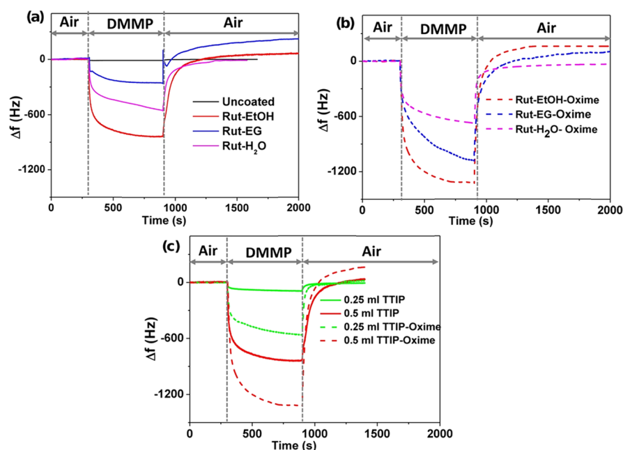
Figure 9. Measured resonant frequency responses for exposition to 500 ppm of DMMP vapor for (a) cantilevers prepared in 0.5 mL of TTIP and a solvent (ethanol, ethylene glycol, or water) and pristine microcantilever and (b) oxime-functionalized cantilevers. (c) Cantilevers prepared in 0.25 and 0.5 mL of TTIP.
