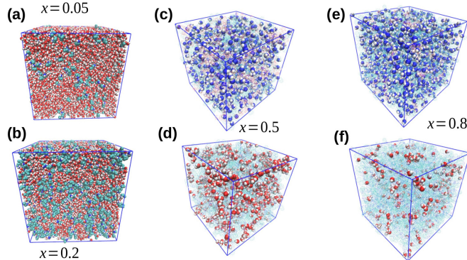
Figure 2: Snapshots of aqueous propylamine mixtures for various propylamine mole fractions x displayed near each panels. (a) x=0.05 (for 16000 molecules); (b) x=0.2 (for 16000 molecules); (c) and (d) for x=0.5 (2048 molecules); (e) and (f) for x=0.8 (2048 molecules). For these 2 latter concentration, upper panels (c) and (e) highlight the amine groups, while lower panels (d) and (f) highlight the water molecules. Omitted atomic groups are shown as semi-transparent. In all snapshots nitrogen atoms are in blue, oxygen in red and hydrogen in white.
