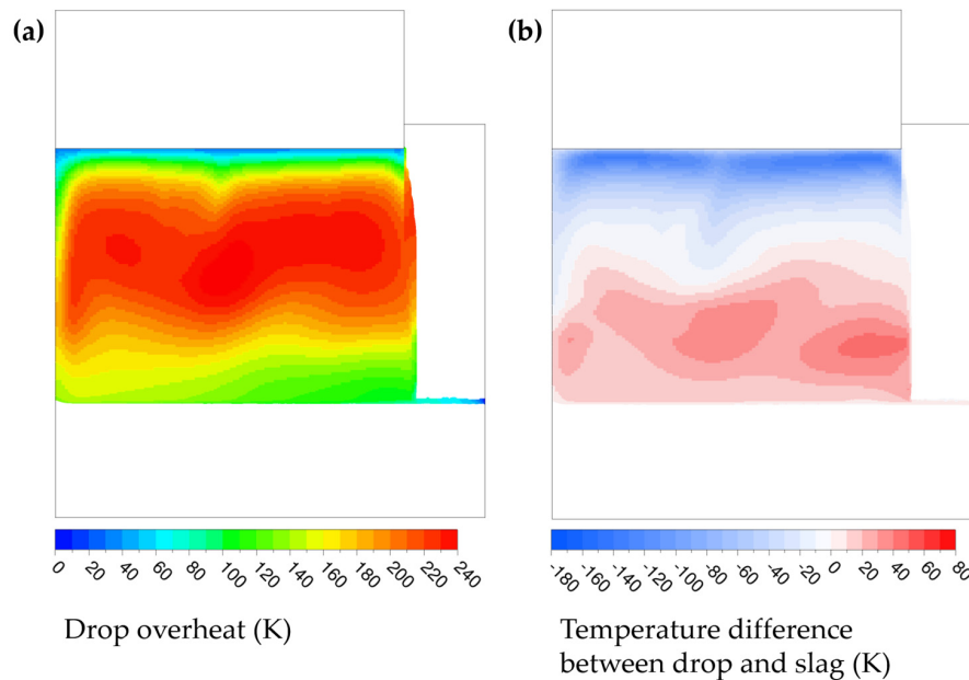
Figure 8. Drop overhear (a) and temperature difference between the drops and the slag (b) (time-averaged) for the 5 mm falling drops.
