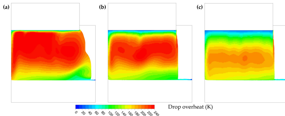
Figure 14. Drop overheating (time-averaged) considering the fall of 1 (a), 5 (b) and 10 mm (c) drops.
