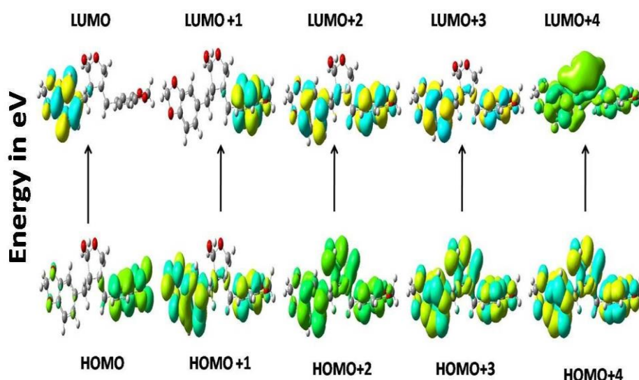
Figure 7: Schematic diagram of the NTO's of Cubecubin calculated at the 6-311++G** level of theory. The surfaces are generated with an isovalue at 0.02
