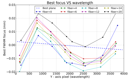
Figure 4. Blue channel on SM9: best plane defocus determination as a function of fiber (left) or wavelength (right), from first scan data (top) and after tilt correction scan data (bottom)
