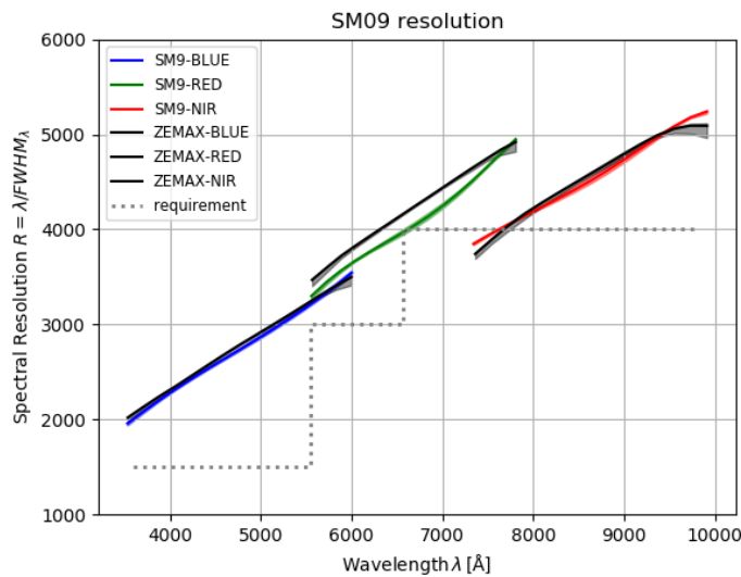
Figure 11 : SM9 resolution (in blue, green and ref for b, r and z channels) based on arc lamp exposures. To be compared with model (black).
