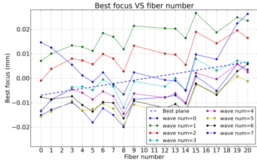
Figure 4. Blue channel on SM9: best plane defocus determination as a function of fiber (left) or wavelength (right), from first scan data (top) and after tilt correction scan data (bottom)
