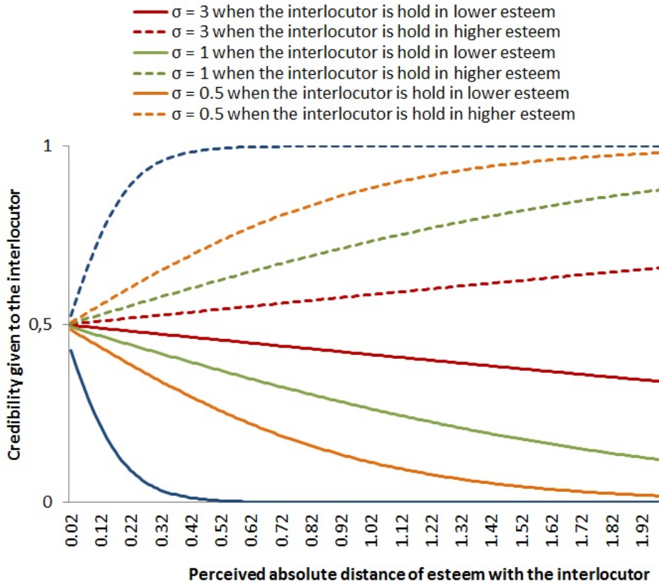
Figure 5. Examples of credibilities (i.e. strength of the influence) given by an agent i to an agent interlocutor j depending on the absolute perceived distance i between j and him-herself (on the x-axis), and the fact i hold j in lower esteem (plain lines) or higher esteem (dotted lines), for \sigma = 0.1 (in blue), 0.5 (in orange), 1 (in green) and 3 (in red). We observe that the higher the perceived distance, the lower the credibility for j when held in lower esteem, or the higher credibility for j when held in higher esteem. Moreover, the larger \sigma , the smaller the difference of given credibility to j if he/she is held in low compared to high esteem.
