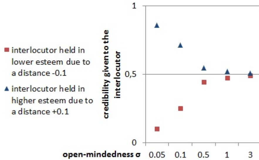
Figure 6. Credibility given to an interlocutor for whom our esteem varies around our self-esteem by 0.1 for different values of the open-mindedness \sigma ; for a variation of: -0.1 implying the interlocutor is held in lower esteem (red square), or +0.1 implying the interlocutor is held in higher esteem (blue triangle).
