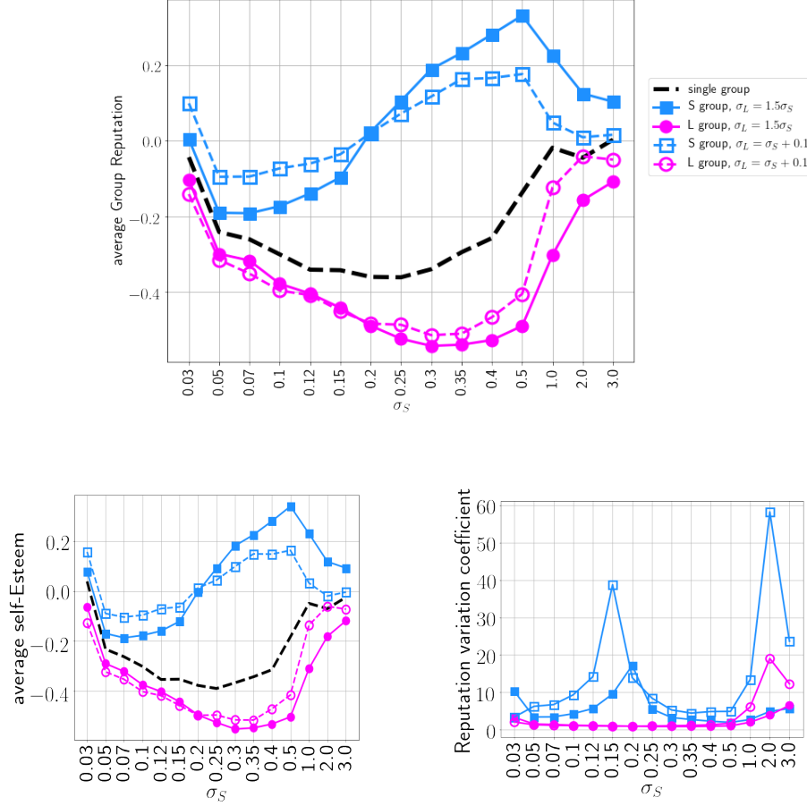
Figure 2. Upper plot: average group reputation for different values of \sigma_S . Lower left plot: average self-esteem of the groups for different values of \sigma_S . Lower right plot: Intra-group variability - variation coefficient for different values of \sigma_S . The black baseline represents a single group with open-mindedness parameter \sigma_S . In the other cases the population is divided into two equal-size groups with open-mindedness parameter \sigma_S (blue lines) and \sigma_L = f(\sigma_S) (magenta lines). The empty symbols correspond to the function: \sigma_L = \sigma_S + 0.1 the others to the case \sigma_L = 1.5\sigma_S
