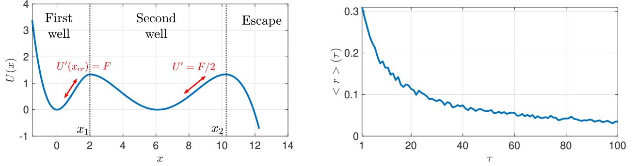
Figure 4: Left: The metastable potential U(x) . The AOPU particle has to cross two barriers at x_1 and x_2 to escape. The two wells are designed such that the maximal slope of the first barrier is F , whereas the maximal slope of the second is F/2 . Right: The graph displays the average fraction of time \langle r \rangle [defined in Eq. (33)] spent by the particle in the second well, as a function of \tau . When \tau becomes large, the particle just jumps ballistically over the second well and escape. Thus \langle r \rangle goes to zero for large \tau .
