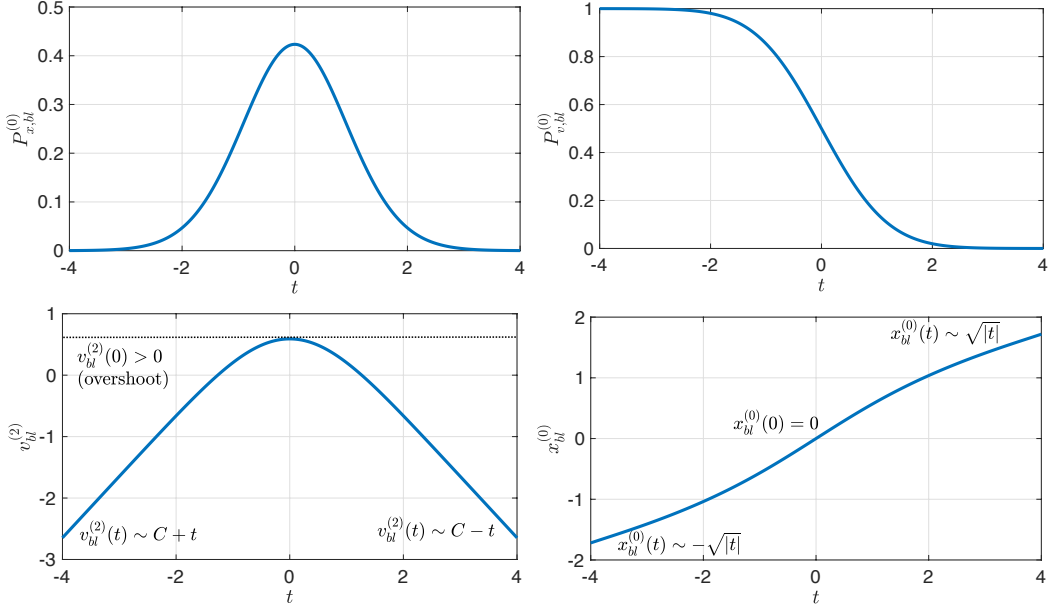
Figure 5: Numerical resolution of the undimensioned boundary layer equations Eqs. (72-73).
