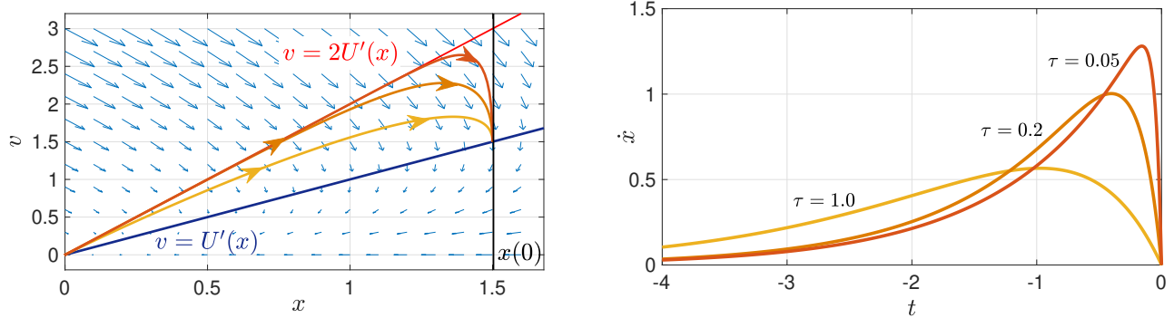
Figure 1: Fluctuation path for the AOUP in a harmonic potential U(x) = \frac{x^2}{2} . Left: The graph displays the fluctuation paths in the phase space (x, v) , for the three values \tau = 1.0/0.2/0.05 . The light blue arrows represent the vector field for \tau = 0.5 . The dark blue line gives the conditions for spatial stationary state \dot{x} = 0 , and the red line is the equation v = 2U'(x) for the equilibrium fluctuation path ( i.e. \tau = 0 ). It can be seen that the convergence to the equilibrium path in the limit \tau \rightarrow 0 displays a singularity close to x(0) = 1.5 . Right: The trajectories \dot{x}(t) for the same values of \tau as in the left picture. The fluctuation path satisfies \dot{x}(0) = 0 , whatever the value of \tau . The boundary layer of size \propto \tau can clearly be identified close to t = 0 .
