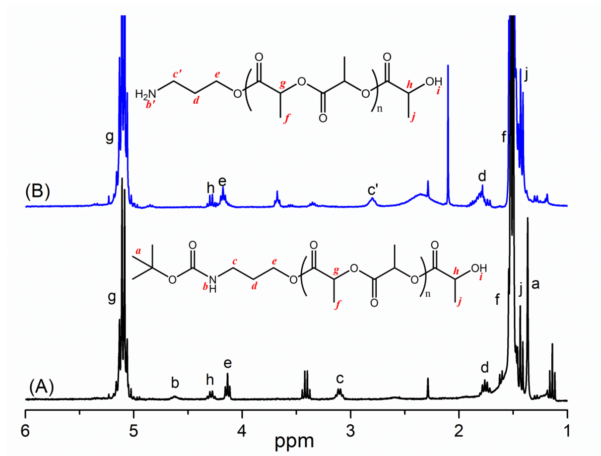
Fig. 1. NMR spectra of Boc-NH-PLA (A) and NH 2 -PLA (B) in CDCl 3 .
