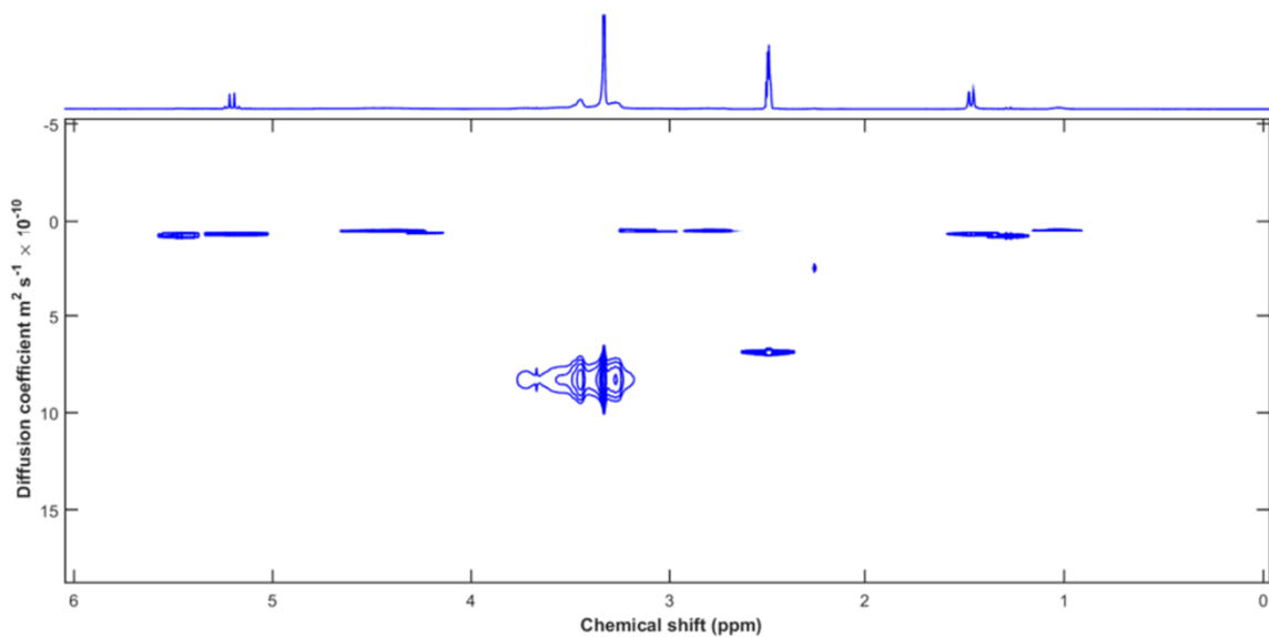
Fig. 3. DOSY- NMR spectrum of HPMC-PLA 10 in DMSO- d 6 .
