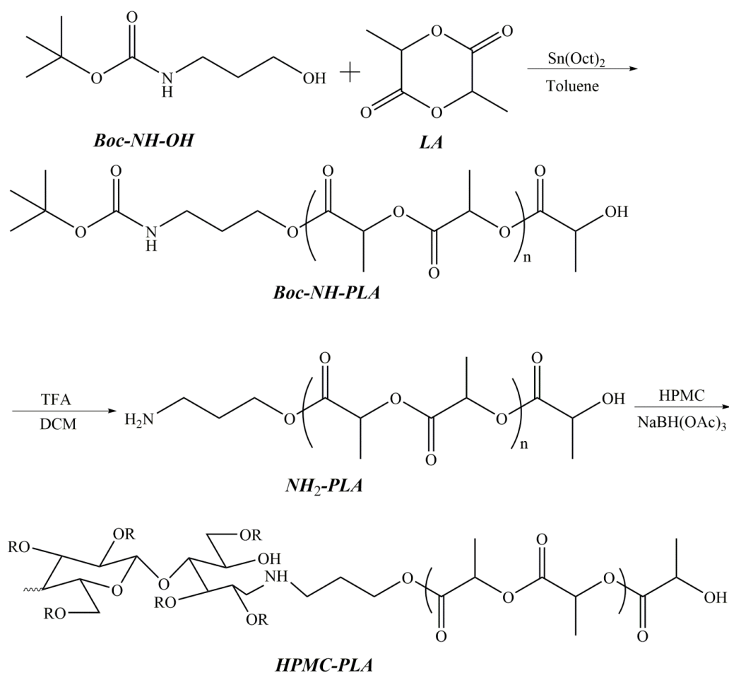
Scheme 1. Synthesis route of HPMC-PLA block copolymers by reductive amination.
