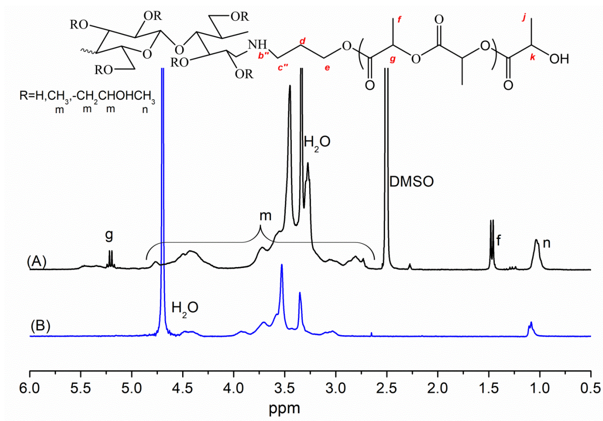
Fig. 2. 1 H NMR spectra of HPMC-PLA in DMSO- d 6 (A) and D 2 O (B) .
