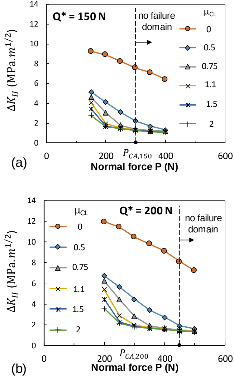
Figure 11: \Delta K_{II} at the crack tip as a function of the normal force, for various friction coefficients \mu_{CL} between the crack lips; (a) for Q^*=150 \text{ N} and \sigma_{f,max} = 60 \text{ MPa} ; (b) for Q^*=200 \text{ N} and \sigma_{f,max} = 60 \text{ MPa}
