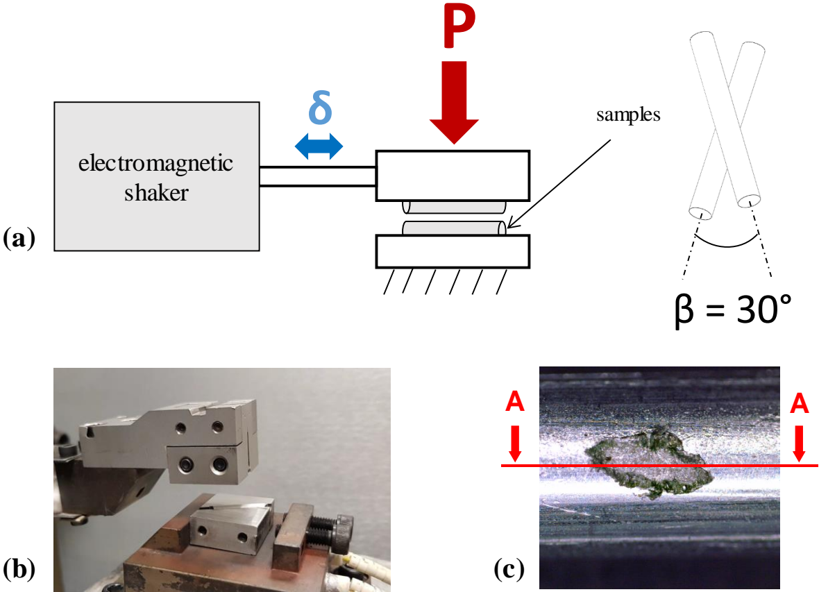
Figure 3: (a) Schematic drawing of the plain fretting test bench used ; (b) picture of the sample holders of the corresponding bench; (c) elliptical fretting scar induced by partial slip conditions displayed with a typical cutting plane used for crack length measurements ( Q^* = 100\text{N} , P = 150\text{N} , N=3 \cdot 10^5 cycles)
