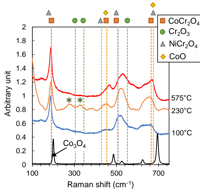
Fig. 7: Raman spectra of wear track at 100°C, 230°C and 575°C. Reference lines and the Co 3 O 4 spectra are extracted from [6].
