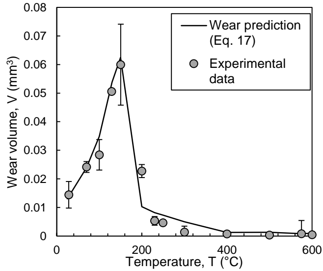
Fig. 14: Comparison between experiments and theoretical calculation for various temperatures (the other parameters are fixed to their reference)
