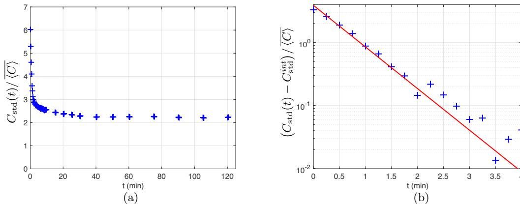
FIG. 3: (a) Temporal evolution of the concentration field standard deviation: C_{\text{std}}(t) = \sqrt{\langle C^2 \rangle - \langle C \rangle^2} , normalized by the global mean \langle C \rangle in the case of N = 15 swimmers with radius R = 2.5 mm. (b) Short term evolution of (C_{\text{std}}(t) - C_{\text{std}}^{\text{int}})/\langle C \rangle plotted in semilog representation, with C_{\text{std}}^{\text{int}}/\langle C \rangle = 2.7 . For those figures the points are obtained with a sliding window average over a few seconds, so that the error is very low.
