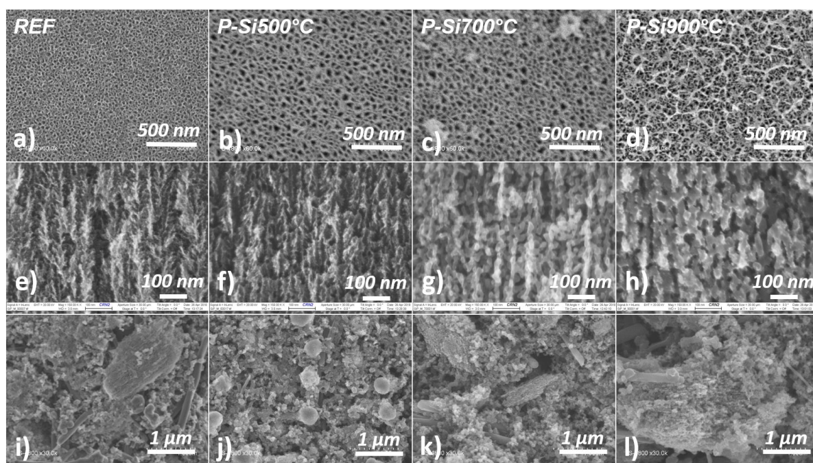
Figure 1: SEM image of a) PSi(REF) ,b) PSi(500°C), c) PSi(700°C), d) PSi(900°C) from top of the film ; Cross section of e) PSi(REF) ,f) PSi(500°C), g) PSi(700°C), h) PSi(900°C) ; Electrode view of i) PSi(REF) ,j) PSi(500°C), k) PSi(700°C), l) PSi(900°C)
