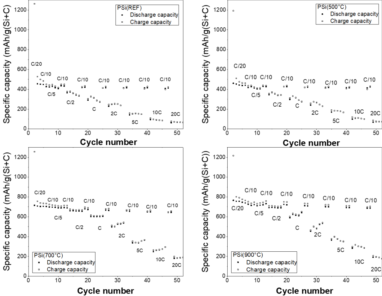
Figure 6 : Variable Current-rate measurements - 0.01-1.5V Vs Li + /Li
