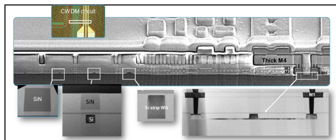
Fig.1: 300mm Si Photonic Platform including Si & SiN waveguides, adiabatic transition, Thick M4 Cu level and Deep Rib HSPM modulators. Integrated Ge PD is not shown on the picture.
