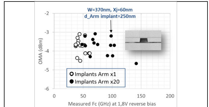
Fig 6: Confirmation of best geometry confirmed with cut-off frequencies measured at 1,8V reverse bias on dedicated RF structures. L=2,4mm.
