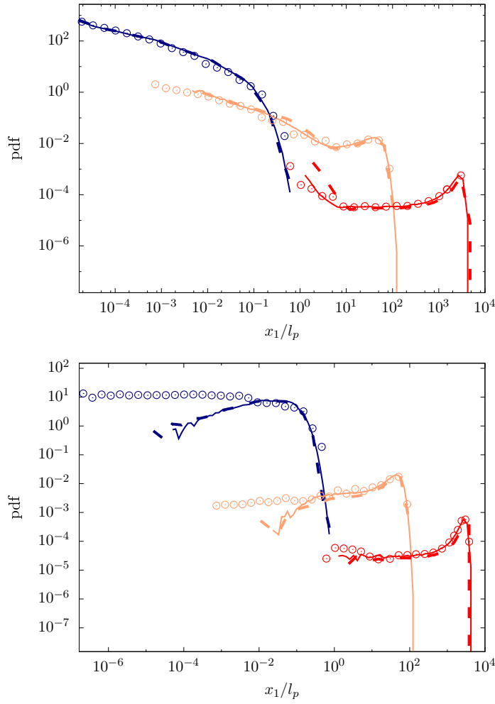
Fig. 5 Evolution of the DNS (circles), OU model (solid lines), and Bernoulli model (dashed lines) mean flow direction propagators for (top panel) uniform injection and (bottom panel) flux-weighted injection at times t = 3.5 \cdot 10^{-1} \tau_c (blue), t = 3.5 \cdot 10^2 \tau_c (orange), and t = 3.5 \cdot 10^4 \tau_c (red).
