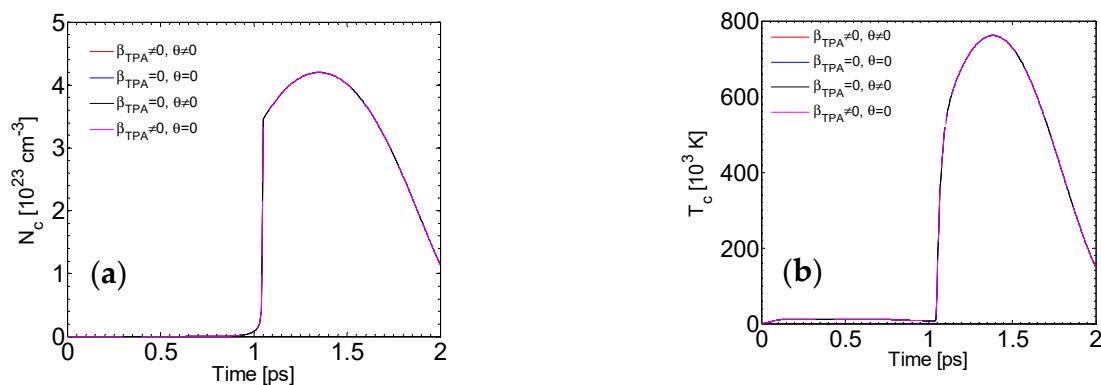
Figure A2. Simulation results of maximum carrier density (a) and carrier temperature (b) for t_{delay} = 0 ps, E_p = 50 mJ/cm 2 for (100) TiO 2 .
