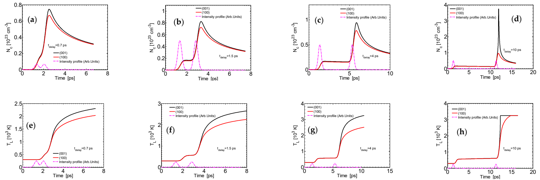
Figure 7. Evolution of maximum carrier density (first row) lattice temperature (second row) for t_{\text{delay}} = 0.7 ps (a,e), 1.5 ps (b,f), 4 ps (c,g) and 10 ps (d,h), respectively. ( E_p = 10 \text{ mJ/cm}^2 ) for (001) and (100) crystal orientation.
