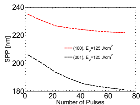
Figure 9. SPP wavelength vs. NP . ( t_{delay} = 4 ps, E_p = 125 mJ/cm 2 for (100) and (001) TiO 2 ).
