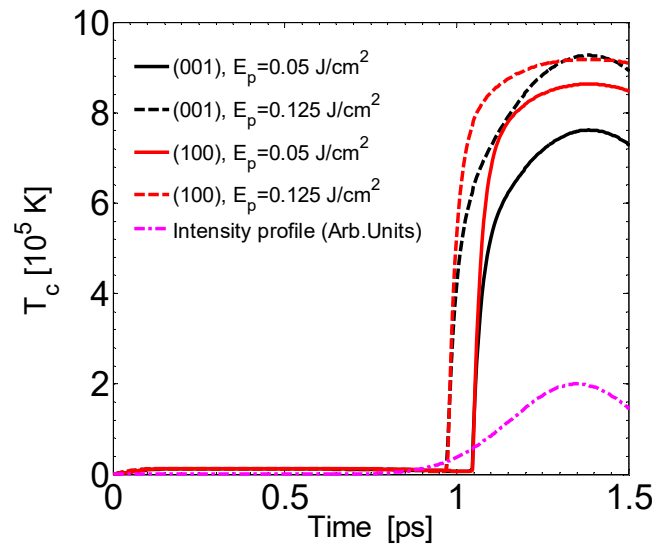
Figure A1. Evolution of values of carrier for E_p = 50 mJ/cm 2 and 125 mJ/cm 2 for (001) and (100) crystal orientation at x = y = 0 and on the surface of the material.
