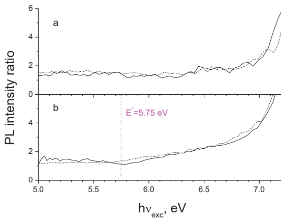
Fig. 8. Intensity ratio of PLE spectra before and after irradiation of \text{MgAl}_2\text{O}_4 ceramics without (a) and with 1 wt% \text{Ta}_2\text{O}_5 (b): UV2 band (F-centres, solid line) and V1 band ( F^+ -centres, dashed line) ( T=9 K).
