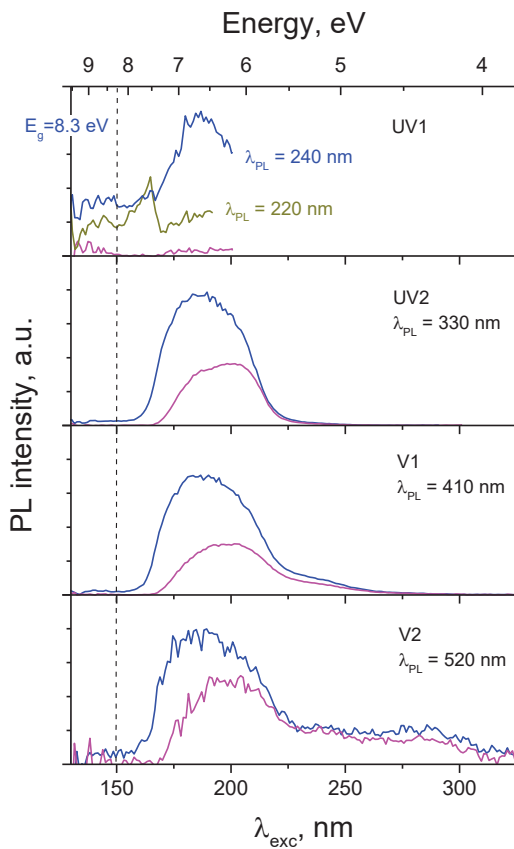
Fig. 7. PLE spectra of MgAl_2O_4 ceramics with 1 wt% Ta_2O_5 before (blue, gray) and after (magenta) He^+ irradiation. PL bands and respective wavelengths are indicated ( T=9 K).
