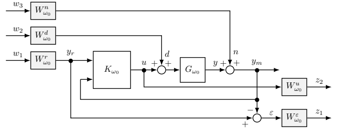
Fig. 1. H_\infty criterion.
