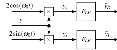
Fig. 2. Block-diagram of the synchronous demodulation.
