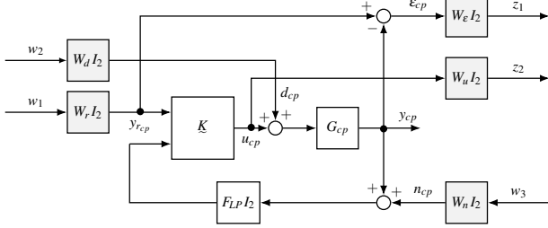
Fig. 4. Considered criterion for the H_\infty synthesis.
