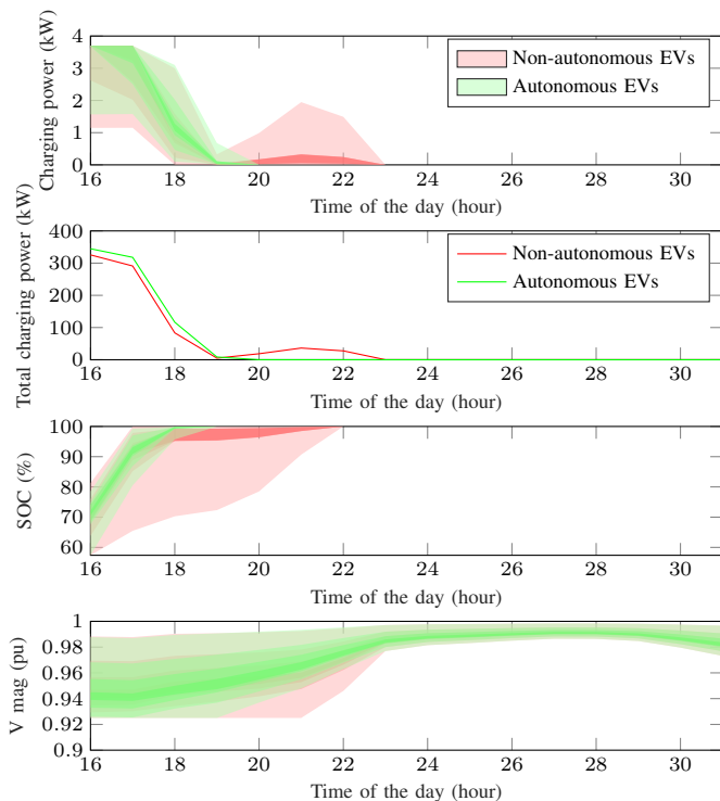
Fig. 4. Charging power (first panel), total charging power, and SOC (third panel) of the EVs population, and nodal voltage magnitude (fourth panel) of all grid nodes. In the 1st, 3rd, and 4th plots, the lighter color-shade refers to the 0 and 1 quantiles, the thicker to the 0.43 and 0.57 ones, whereas the two primary colors red and green refer to conventional and autonomous EVs, respectively.
