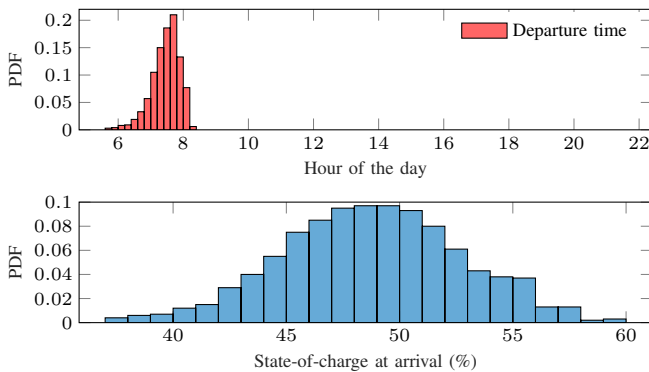
Fig. 3. Distributions of the EVs' departure times (upper-panel plot) and of the initial SOC (lower-panel plot) used in the simulations.
