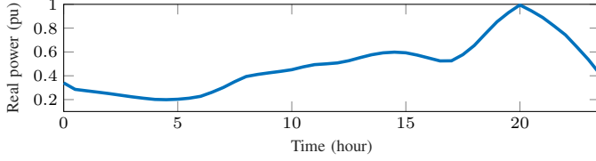
Fig. 2. Profile of the net active power demand from CIGRE specifications [19].
