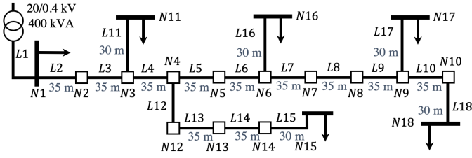
Fig. 1. Topology of European LV distribution network benchmark for residential system used for the verification [19].
