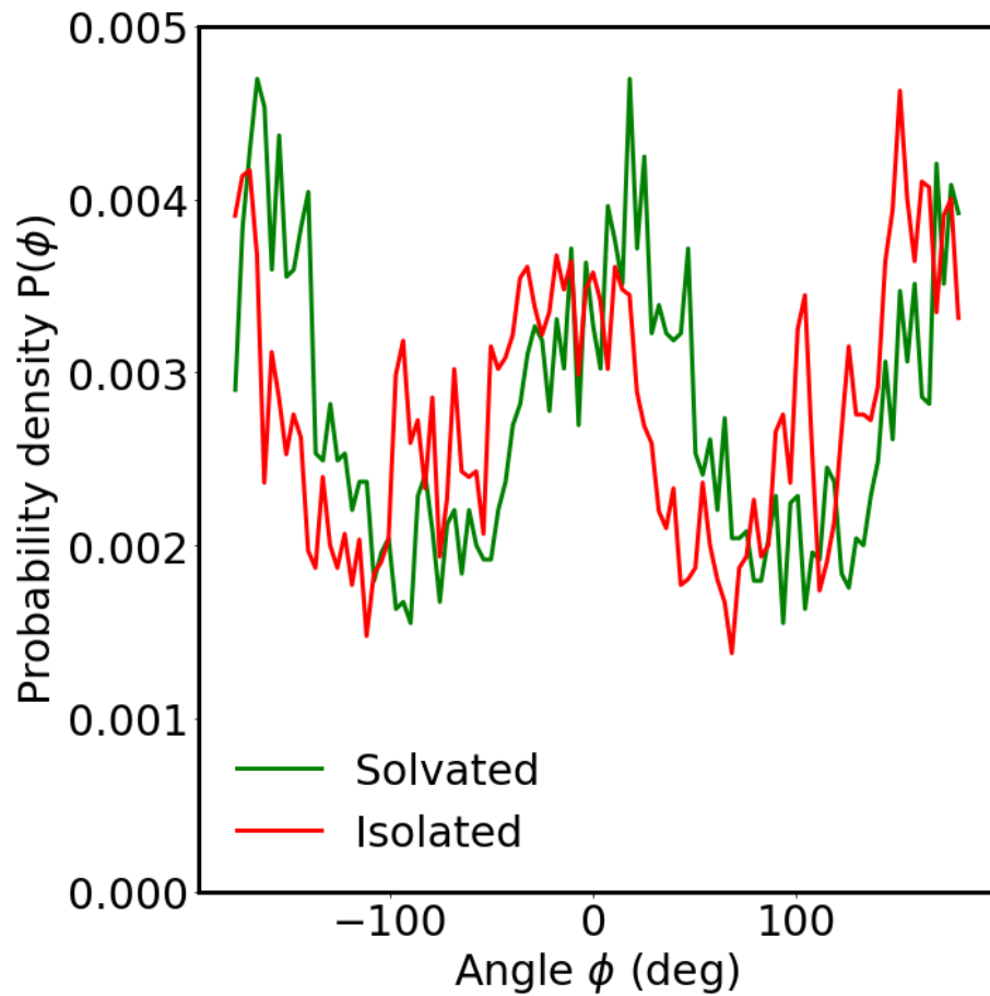
Figure 5: Distribution of O-C-O*-C dihedral angle of pyrocarbonate C_2O_5^{2-} solvated in the eutectic LiKCO_3 at 1000 K and isolated. For the solvated molecule, the dihedral angle is measured during the time intervals of existence of C_2O_5^{2-} .
