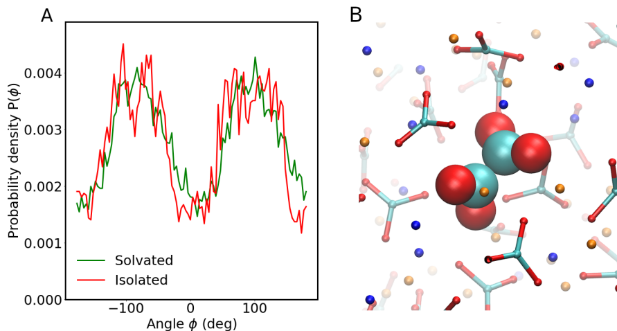
Figure 7: (a) Distribution of O-C-C-O dihedral angle of oxalate C_2O_4^{2-} solvated in the eutectic LiKCO_3 at 1000K and isolated. (b) Snapshot of C_2O_4^{2-} in the eutectic LiKCO_3 . Carbonate molecules in the solvent are represented by cyan/red sticks, O atoms by red spheres, K atoms in blue and Li atoms in orange.
