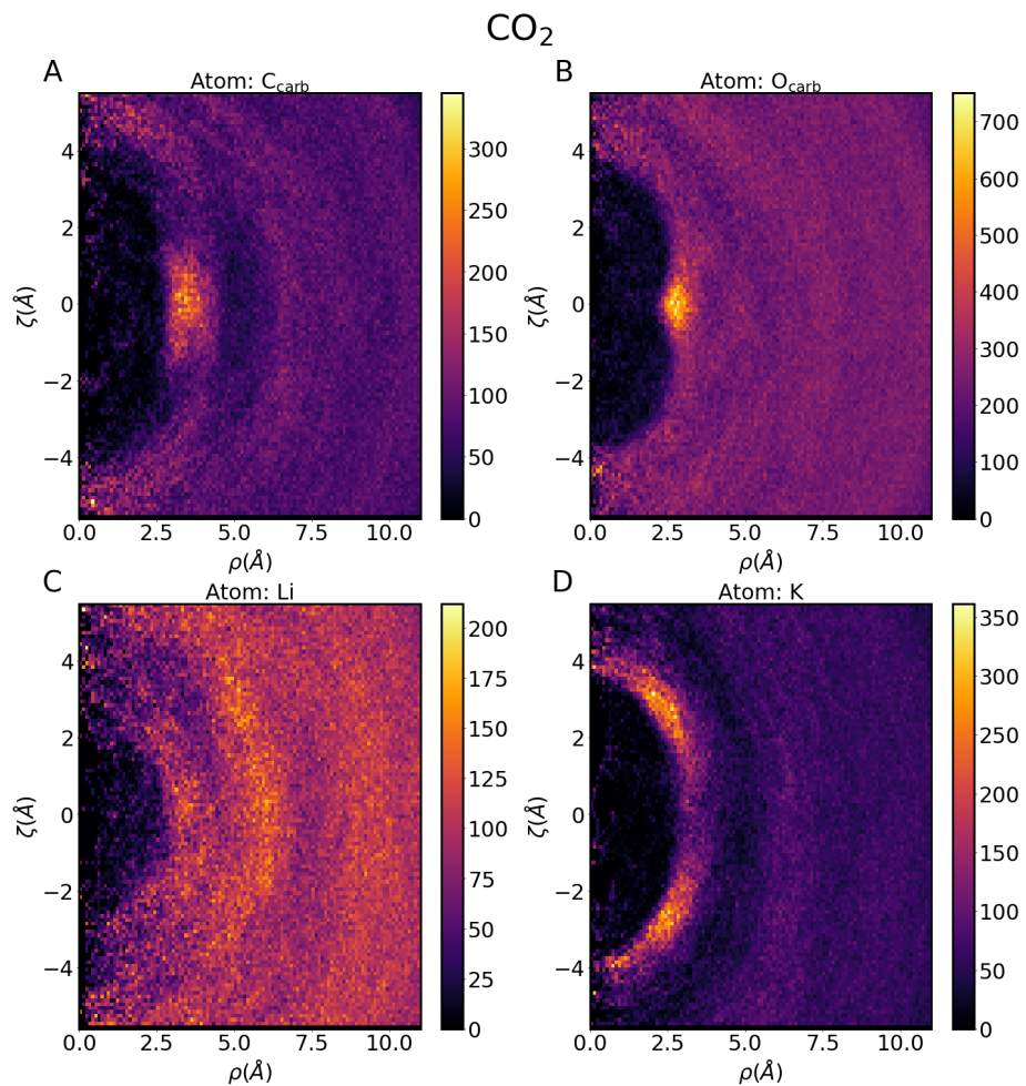
Figure 4: Solvation structure around the CO 2 molecule. Two dimensional colour charts representing the probability of the presence of the following atoms around CO 2 : C carb atom (a); O carb atom (b); Li atom (c) and K atom (d). CO 2 is oriented with its O CO 2 -O CO 2 axis along the \hat{\zeta} direction, where \zeta = 0 is the mid-point of the O-O distance. \zeta is thus the projection of an atom position along the O CO 2 -O CO 2 axis, and \rho its distance from the O CO 2 -O CO 2 axis.
