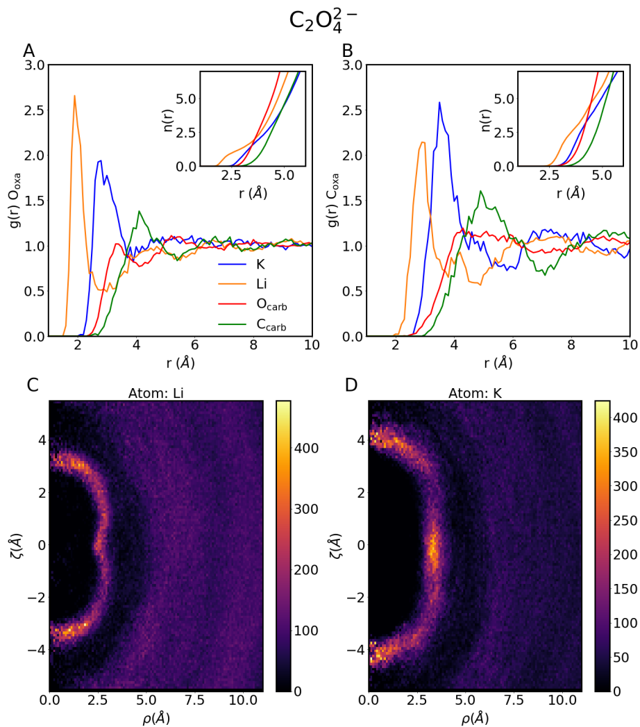
Figure 8: Solvation structure around the oxalate \text{C}_2\text{O}_4^{2-} anion. Upper panel: radial distribution function (RDF) for (a) carbon atom of \text{C}_2\text{O}_4^{2-} and (b) oxygen atom of \text{C}_2\text{O}_4^{2-} . Insets: coordination number n(r) obtained from the integration of the radial distribution functions. The same color code applies for figures (a) and (b). Lower panel: two dimensional colour charts representing the probability of the presence of the following atoms around \text{C}_2\text{O}_4^{2-} : Li atom (c) and K atom (d). \text{C}_2\text{O}_4^{2-} is oriented with its \text{C}_{\text{oxa}}-\text{C}_{\text{oxa}} axis along the \hat{\zeta} direction, where \zeta = 0 is the mid-point of the \text{C}_{\text{oxa}}-\text{C}_{\text{oxa}} distance. \zeta is thus the projection of an atom position along the \text{C}_{\text{oxa}}-\text{C}_{\text{oxa}} axis, and \rho its distance from the \text{C}_{\text{oxa}}-\text{C}_{\text{oxa}} axis.
