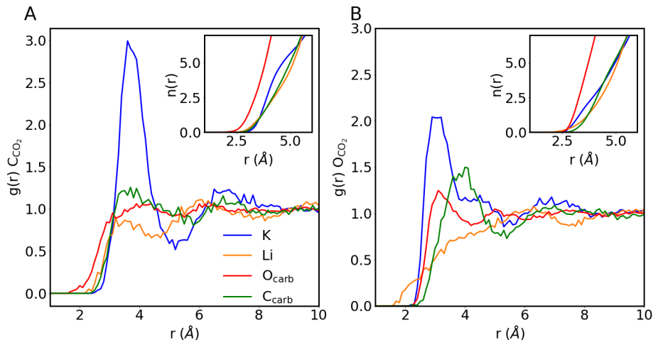
Figure 3: Radial distribution function (RDF) around the (a) oxygen atom of CO 2 molecule O_{CO_2} and (b) carbon atom of CO 2 molecule C_{CO_2} . Intermolecular distances are measured during the time of existence of CO 2 as a molecular species. Insets: coordination number n(r) obtained from the integration of the radial distribution functions. The same color code applies for figures (a) and (b).
