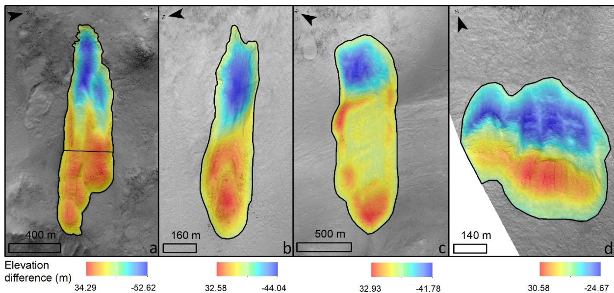
Figure 2: Thickness map of four martian landslide in Nili Fossae region calculated using the methods in Conway and Balme [13]. Black line in (a) show where the cross profile was taken for figure 1. (a) HiRISE image ESP_027480_2075; (b), (c), (d) HiRISE image ESP_027480_2075.
