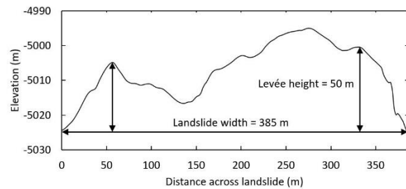
Figure 1: Cross-section of a martian landslide showing the average structure of the levees.
