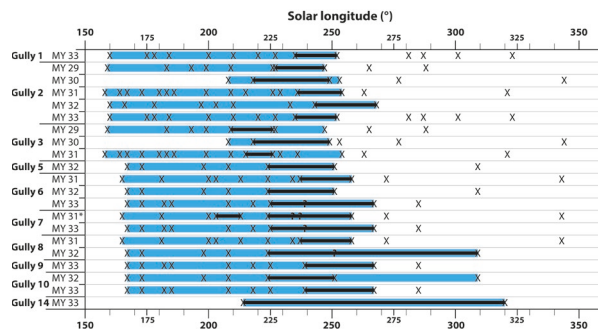
Fig. 3: Diagram of the 10 active gullies with visible changes within one MY. Six of the 10 gullies show periodic activity within different martian years (y-axis). The crosses represent single HiRISE images; the blue bars represent the identified surface frost coverage from the beginning of surface frost (beginning of blue bar) to the first image without any identifiable surface frost (end of blue bar). Black bars represent identified activity from between the “before” and “after” HiRISE images [from 1].
