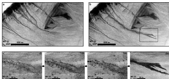
Fig. 1: (a, b) Before and after image of an active gully. (c) A dark flow-like feature formed between Ls 235° and 253° of MY 33 [from 1].
