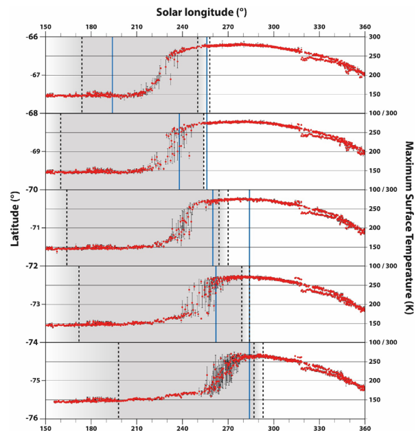
Fig. 2: Diagram of average annual defrosting of the study region in 2° latitudinal bins (left axis) and temperature (right axis) vs. time (end of winter to end of summer). Red dots represent the average of all taken TES maximum daytime surface temperatures at the same time between MY 24 to 26 with standard deviation (black bars). Grey areas represents a fully frosted surface. Surface defrosting took place between the last two dashed lines (based on CTX) and blue lines (based on HRSC) [from 1].
