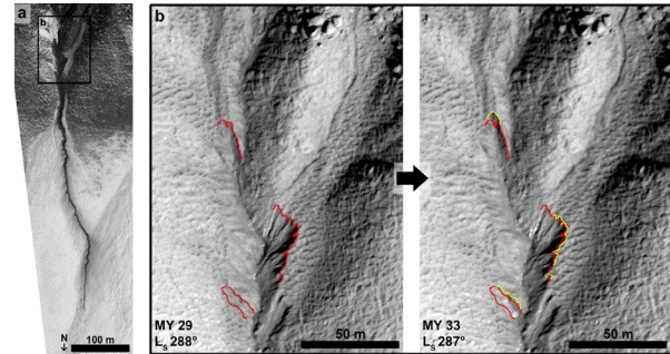
Fig. 4: Headwall erosion of the active gully presented in [2]. (a) Overview image. Before and after images: (b) Detail of gully alcove in MY 29 at L S 288°, red lines represent clearly identifiable outlines of the headwall of the alcove (small active alcove in larger, older and inactive alcove). (c) Erosion of some meters of material in MY 33 (L S 287°), yellow lines represent the new headwall of the alcove [from 1].
