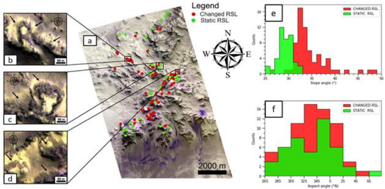
Figure 1 a) CaSSIS color composite of the RED, PAN, and BLU filters showing the location of all identified RSL and their classification in terms of “changed” (red) and “static” (green). b,c,d) Examples of identified RSL as viewed through CaSSIS. e) Slope and f) aspect distributions for “changed” (red) and “static” RSL.
