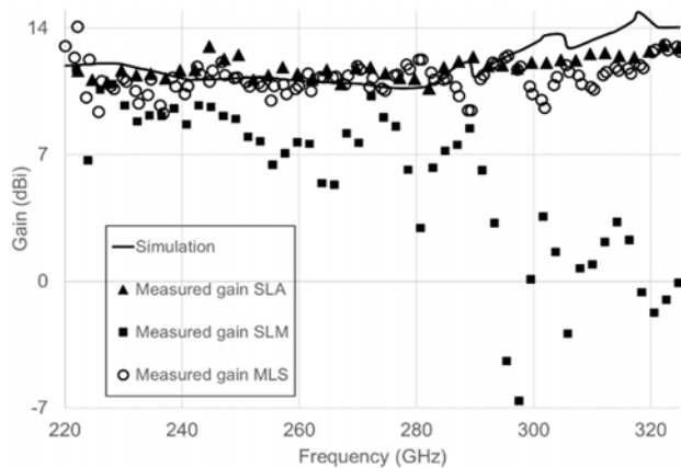
Fig. 8. Simulated broadside horn antenna realized gain and measurements for SLA, SLM and MLS 3D-Printing technologies
