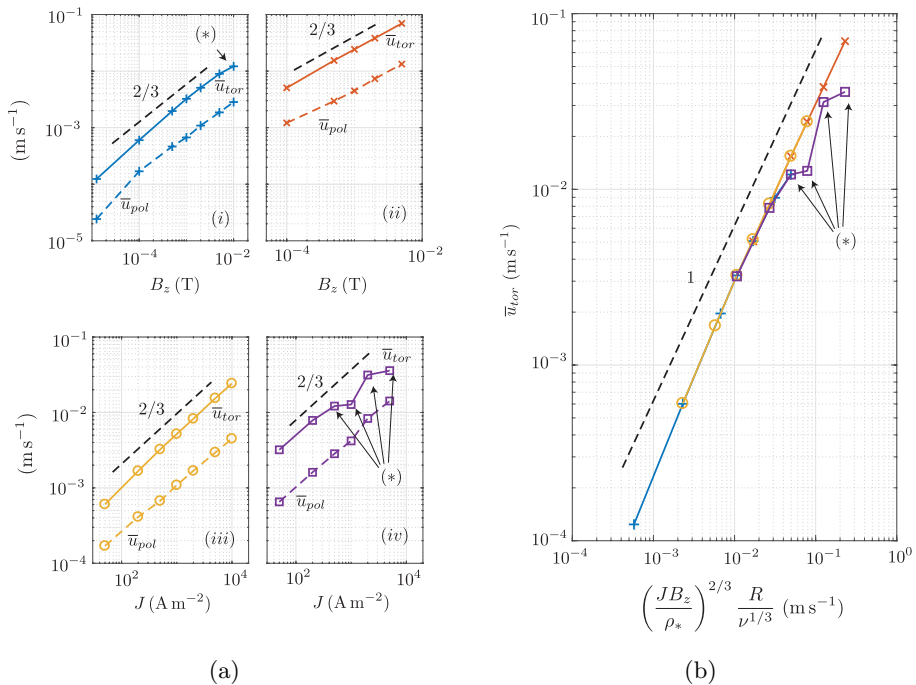
FIGURE 7. Scaling laws for the quantities \bar{u}_{\text{tor}} and \bar{u}_{\text{pol}} using the data sets (i)–(iv) from Table 2. (a) Data set (i) (top left); data set (ii) (top right); data set (iii) (bottom left); data set (iv) (bottom right). (b) \bar{u}_{\text{tor}} as a function of \left(\frac{JB_z}{\rho_*}\right)^{2/3} \left(\frac{R}{\nu^{1/3}}\right) for the combined data sets. The points marked with an asterisk (*) deviate slightly from the scaling law because the induced currents are not negligible.
