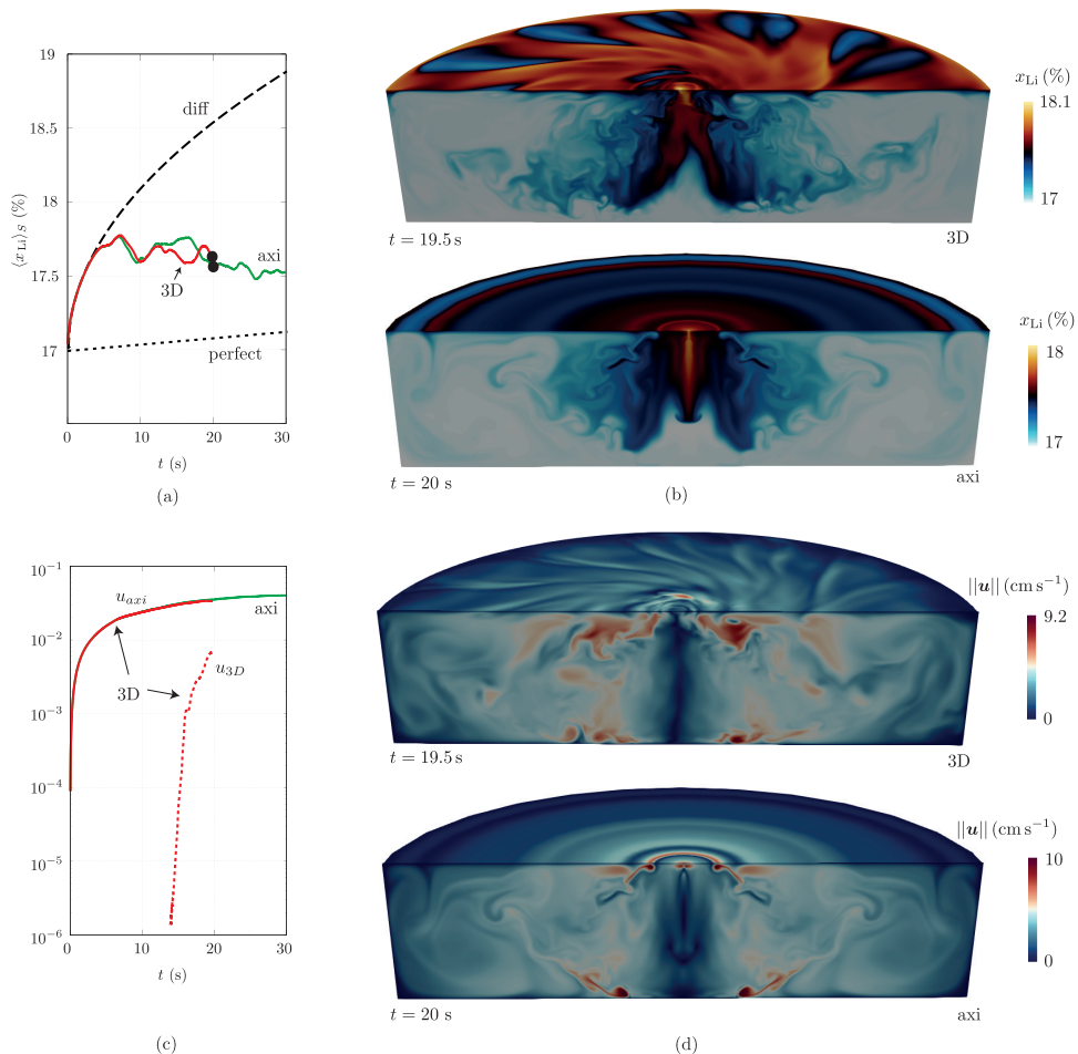
FIGURE 13. Comparison of three-dimensional and axisymmetric simulations for J = -5 \text{ kA m}^{-2} and B_z = -5 \text{ mT} and relaxed D_{\text{relax}} = 8 \times 10^{-8} \text{ m}^2 \text{ s}^{-1} . (a) Surface averaged molar fraction as a function of time. (b) Snapshots of the molar fraction at similar times in x = 0 plane and z = 2 \text{ cm} plane. (c) Rms velocities as a function of time. (d) Snapshots of the flow speed at similar times in x = 0 plane and z = 1.98 \text{ cm} plane.
