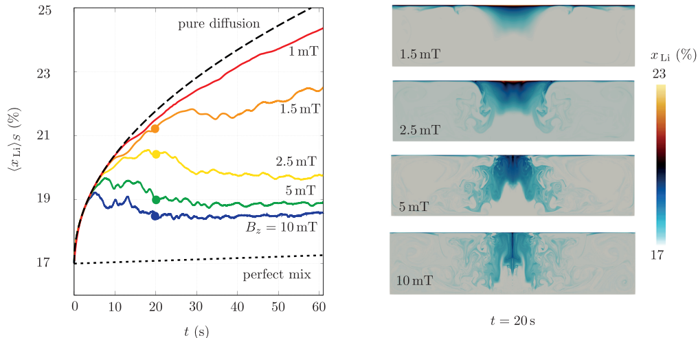
FIGURE 3. Influence of the swirling electrovortex flow on the molar fraction of Li with J = -5 \text{ kA m}^{-2} and B_z \in \{-1, -1.5, -2.5, -5, -10\} mT. (Left) Time evolution of \langle x_{\text{Li}} \rangle_S . The influence of the electrovortex flow is clear for magnetic field intensities greater than |B_z| = 1 mT. (Right) x_{\text{Li}} distribution in the meridian section at t = 20 s.
