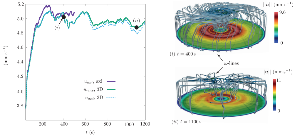
FIGURE 11. Three-dimensional and axisymmetric simulations of the swirling electrovortex flow with J = -1 \text{ kA m}^{-2} and B_z = -1 \text{ mT} . (Left) Time evolution of the rms-velocities u_{axi} and u_{rms} . The axisymmetric and three-dimensional results differ very little. (right) Vorticity lines and magnitude of the velocity in the horizontal plane z = 0.2 \text{ cm} at t = 400 \text{ s} and t = 1100 \text{ s} in the three-dimensional simulation.
