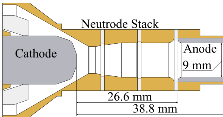
Fig. 1 SimplexPro™ plasma torch scheme
