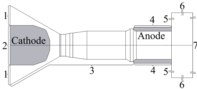
Fig. 4 Boundaries of the computational domain: 1: inlet of plasma-forming gas; 2: rear of the cathode; 3: electrically insulating inter-electrode; 4: rear of the anode; 5 and 6: free boundaries; 7: outlet
