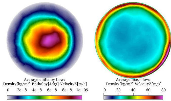
Fig. 17 Enthalpy flow rate and mass flow rate for an external magnetic field of 0.05 T.
