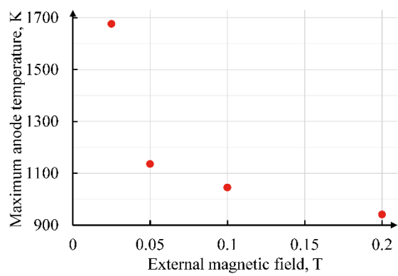
Fig. 16 Variation of maximum anode temperature with the external magnetic field
