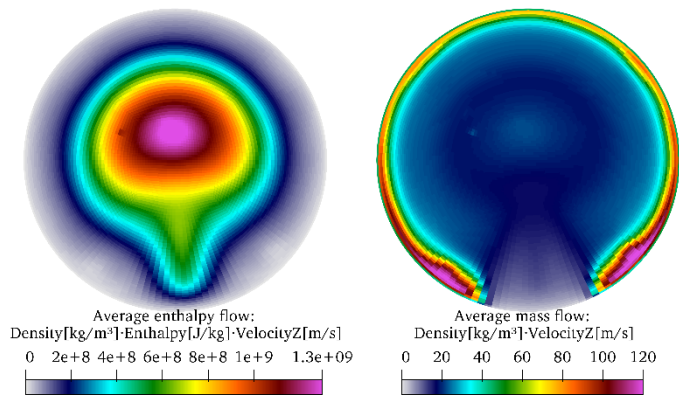
Fig. 10 Enthalpy flow rate and mass flow rate at the nozzle exit. Nozzle \varnothing = 9 mm, 500 A, 60 NLPM Ar. Straight gas injection, no external magnetic field.
