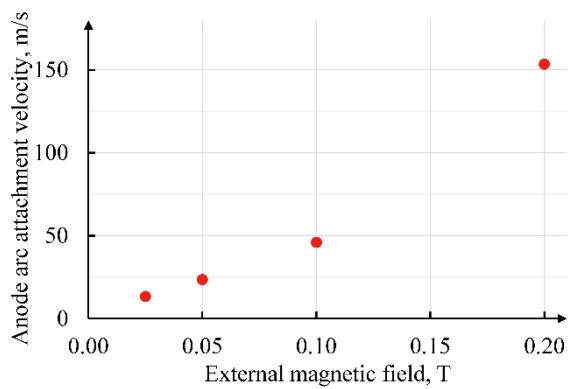
Fig. 15 Variation of the anode arc attachment velocity with the external magnetic field
