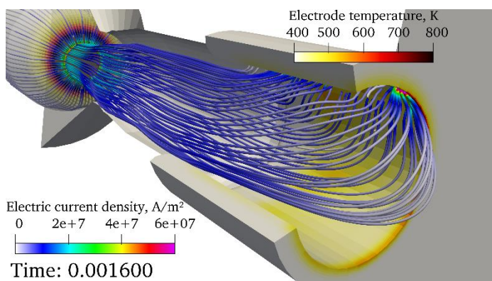
Fig. 12 Anodic arc root movement under the action of an external axial magnetic field of 0.05
