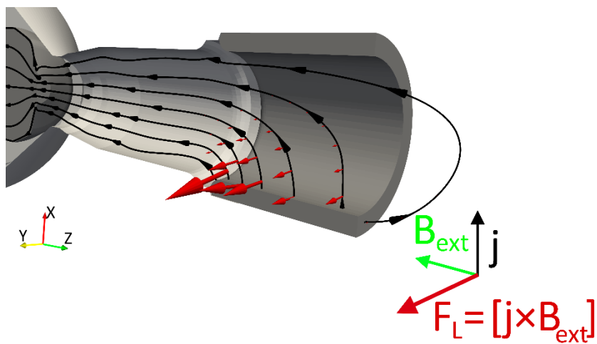
Fig.3. Electric current lines in black and the Lorentz force in red exerted on the moving charge carriers by the external magnetic field in the torch
