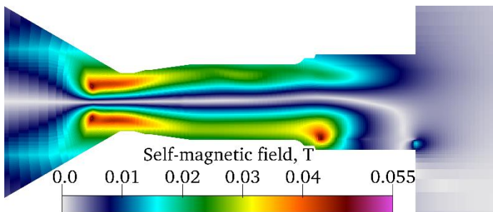
Fig. 11 Self-magnetic field generated by the arc current
