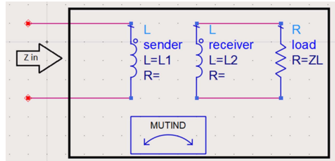
Fig. 7. The circuit model of the transmitter-receiver as a one-port network. By measuring Z_{in} , it is possible to deduce the mutual inductance between the transmitter and the receiver.
