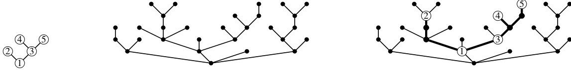
FIGURE 3. Left: a planar rooted labeled tree u . Center: a planar rooted tree t . Right: a proper embedding of u into t .
