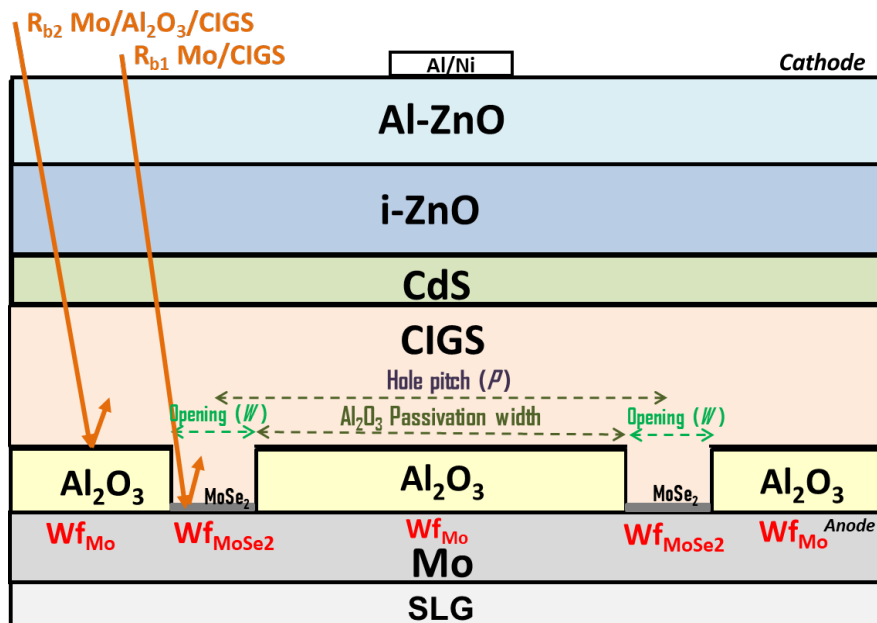
Figure 2: ATLAS 2D ARCIGS-M structure model of \text{Al}_2\text{O}_3 -rear-passivated UT-CIGS cell with openings width (W) and hole pitch (P) including back reflection coefficients ( R_{b1} , R_{b2} ).
