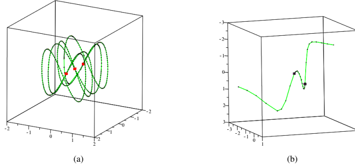
Figure 4: Output of PTOP0 for (a) a Lissajous curve parametrized by (\frac{-t^2-1}{t^2+1}, \frac{-8t(t^2-1)(t^4-6t^2+1)}{t^8+4t^6+6t^4+4t^2+1}, \frac{-(16(t^4-6t^2+1))(t^2-1)t(t^8-28t^6+70t^4-28t^2+1)}{(t^16+8t^14+28t^12+56t^10+70t^8+56t^6+28t^4+8t^2+1)}) . The multiple points are indicated by the red squares. (b) a space curve parametrized by (\frac{-2t^2}{t^2+1}, \frac{-2t(3t^2-19t^4+8t^3-9t^2-t+2)}{(t^2+1)(10t^4-6t^3+3t^2+1)}, t) . The apparent singularities are indicated by the black squares.
