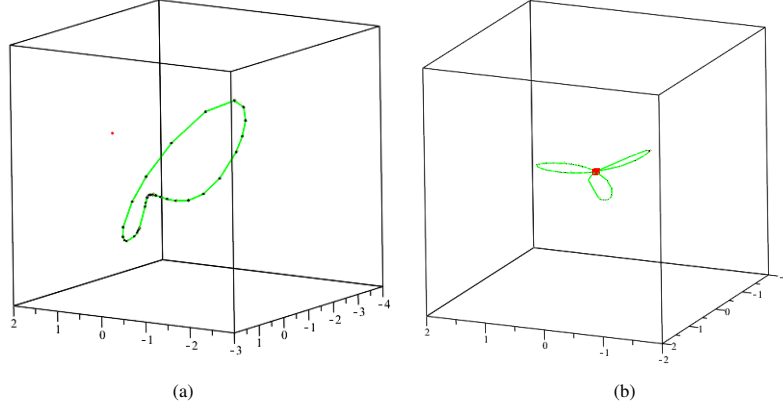
Figure 5: Output of PTOPD for a curve parametrized by (a) \left(\frac{-7t^4+22t^3-55t^2-94t+87}{-56t^4-62t^2+97t-73}, \frac{-4t^4+83t^3-10t^2-62t-82}{-56t^4-62t^2+97t-73}, \frac{-4t^4+83t^3-10t^2-62t-82}{-56t^4-62t^2+97t-73}\right) (b) \left(\frac{-3t^2+1}{(t^2+1)^2}, \frac{(-3t^2+1)t}{(t^2+1)^2}, \frac{(-3t^2+1)t^3}{(t^2+1)^4}\right) . Examples are taken from Alcázar and Díaz-Toca (2010).
