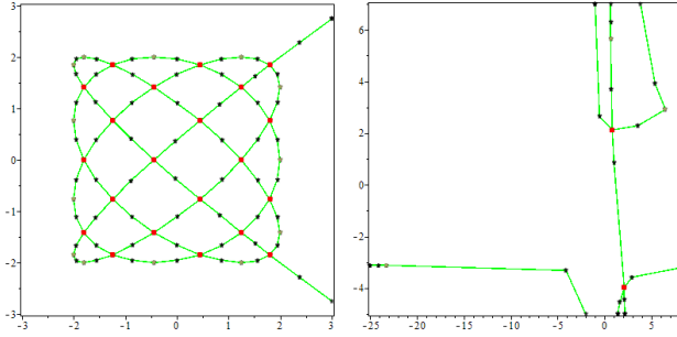
Figure 2: The left figure is the output of \text{PTOP} for the parametric curve (t^8 - 8t^6 + 20t^4 - 16t^2 + 2, t^7 - 7t^5 + 14t^3 - 7t) while the right figure is the output for the curve (\frac{37t^3-23t^2+87t+44}{29t^3+98t^2-23t+10}, \frac{-61t^3-8t^2-29t+95}{11t^3-49t^2-47t+40}) .
