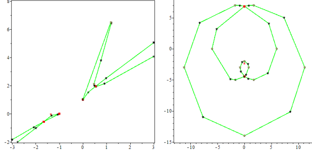
Figure 1: The left figure is the output of \text{PTOP} for the parametric curve (\frac{3t^2+3t+1}{t^6-2t^4-3t-1}, \frac{(t^4-2t+2)t^2}{t^6-2t^4-3t-1}) , while the right figure is the output for the curve (\frac{6t^8-756t^6+3456t^5-31104t^3+61236t^2-39366}{t^8+36t^6+486t^4+2916t^2+6561}, \frac{-18(6t^6-16t^5-126t^4+864t^3-1134t^2-1296t+4374)t}{t^8+36t^6+486t^4+2916t^2+6561}) .
