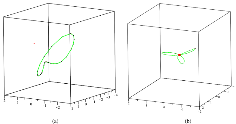
Figure 5: Output of PTOPO for a curve parametrized by (a) (\frac{-7t^4+22t^3-55t^2-94t+87}{-56t^4-62t^2+97t-73}, \frac{-4t^4+83t^3-10t^2-62t-82}{-56t^4-62t^2+97t-73}, \frac{-4t^4+83t^3-10t^2-62t-82}{-56t^4-62t^2+97t-73}) (b) (\frac{-3t^2+1}{(t^2+1)^2}, \frac{(-3t^2+1)t}{(t^2+1)^2}, \frac{(-3t^2+1)t^3}{(t^2+1)^4}) . Examples are taken from Alcázar and Díaz-Toca (2010).
