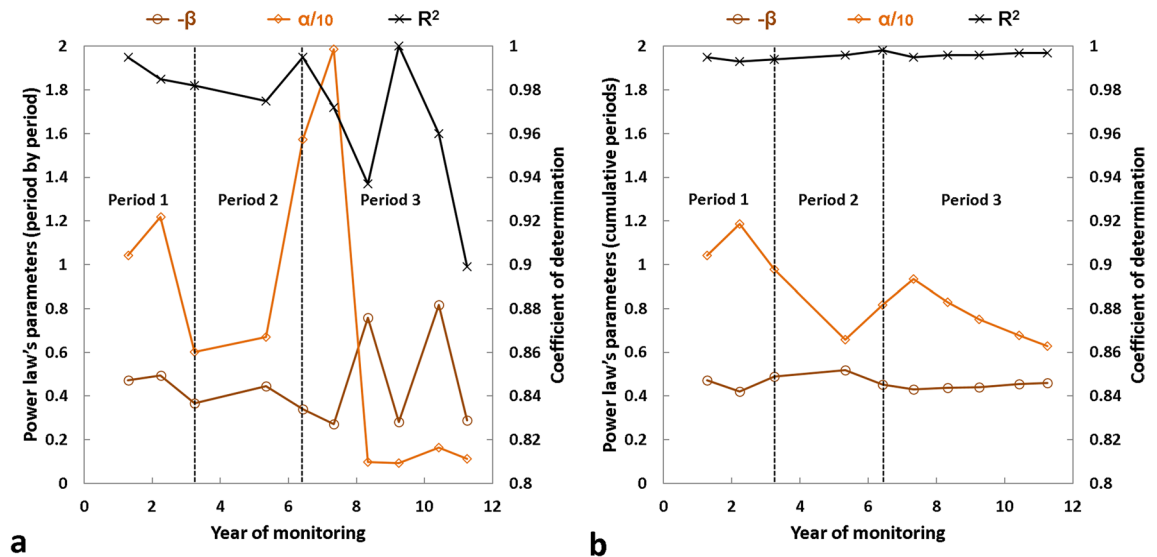
Figure 9. Rockfall source power law statistics determined between 2005 and 2016 in the Drus west face. Temporal evolution of parameters \alpha and \beta and the coefficient of determination R^2 by considering each monitored period as independent (a) or by cumulating the periods (b). The values of \alpha and \beta are on the left y-axis, and the values of R^2 are on the right y-axis; \alpha -values have been divided by ten to appear on the graphs. The domains of validity and goodness-of-fit indicators of each power law are specified in Supplementary Tables 1 and 2, respectively.
