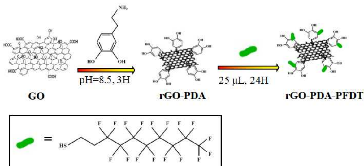
Scheme 1. Schematic illustration of the preparation of rGO-PDA-PFDT.
