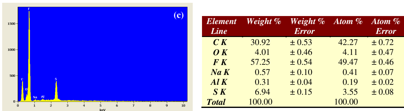
Figure 5. EDX spectra of GO (a), rGO-PDA (b) and rGO-PDA-PFDT (c) membranes.
