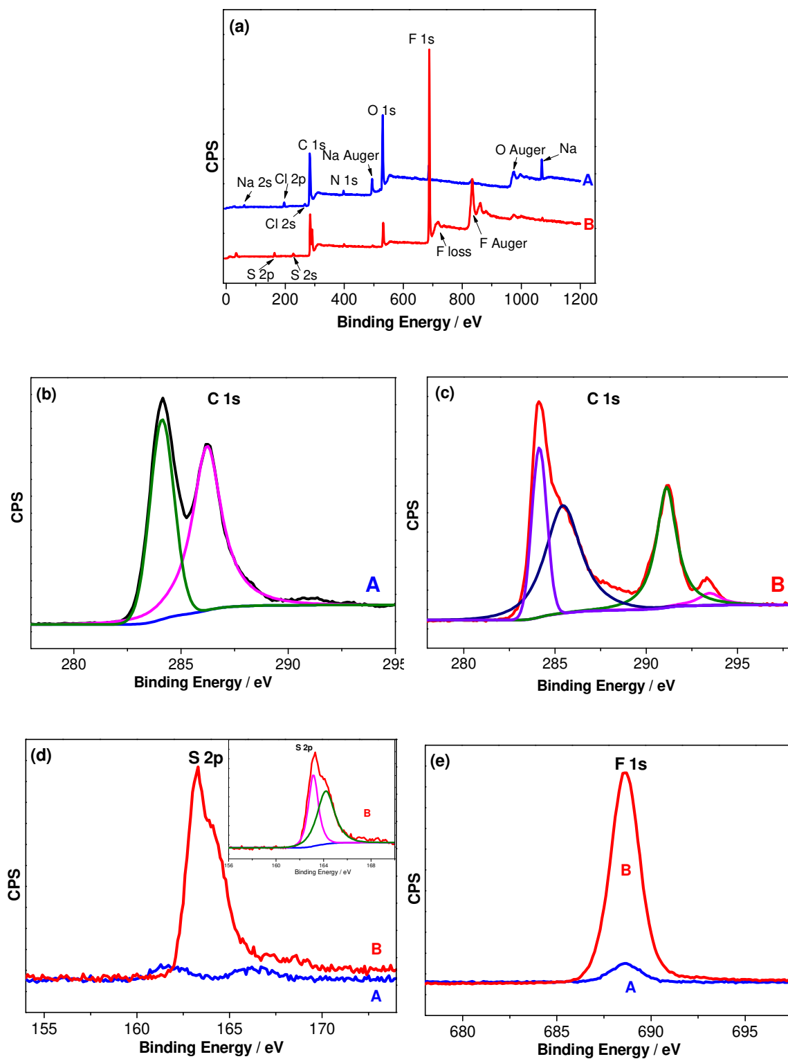
Figure 10. XPS spectra: (a) the survey spectra, (b) fitted curve of C 1s region of sample A, (c) fitted curve of C 1s region for sample B, (d) S 2p region, and the inset is fitted curve of sample B, (e) F 1s region; (A) rGO-PDA (blue line), (B) rGO-PDA-PFDT (red line).
