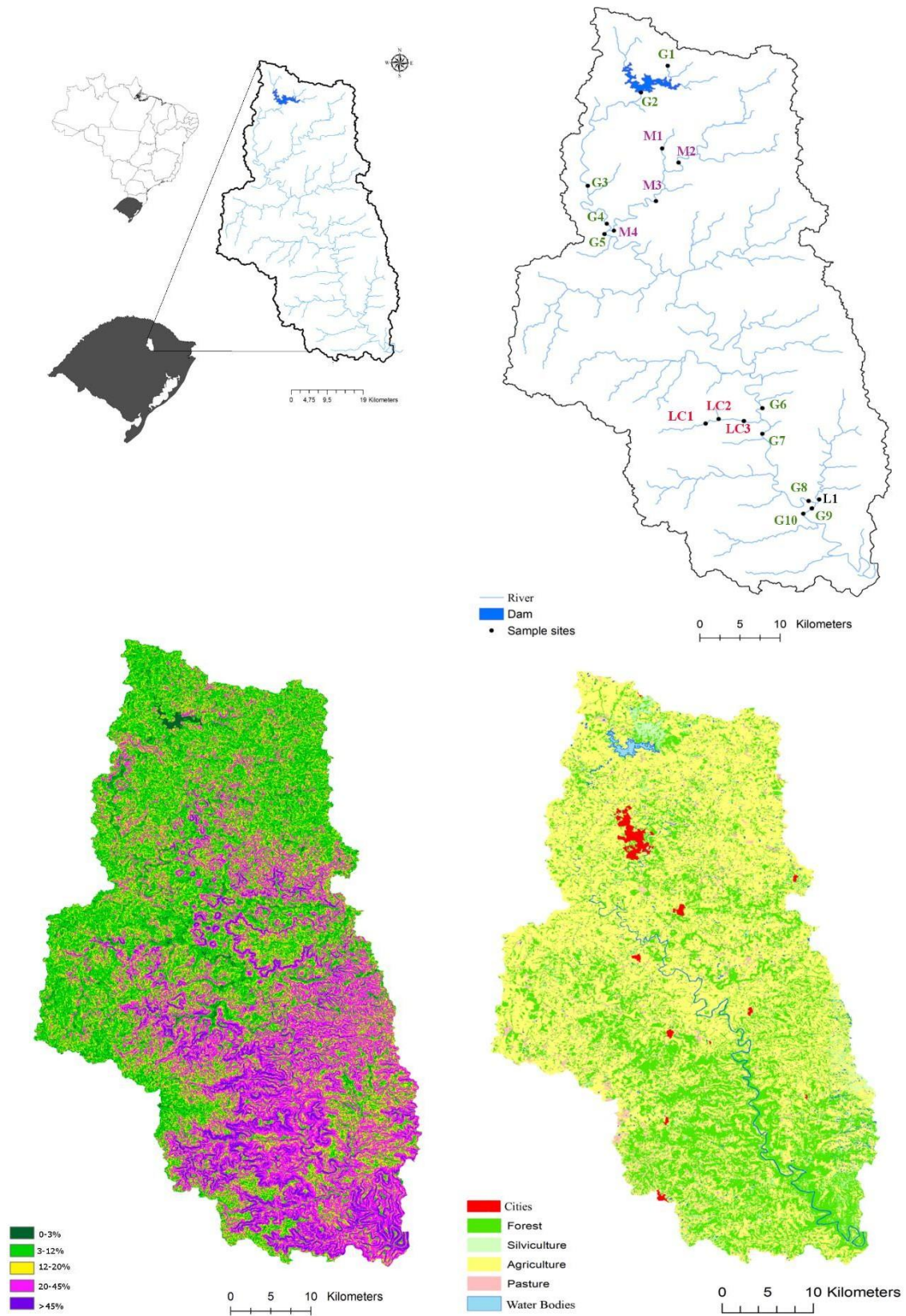
Fig. 1. Characteristics of area and location of the sampling sites in the Guaporé River and its tributaries (RS – Brazil).
