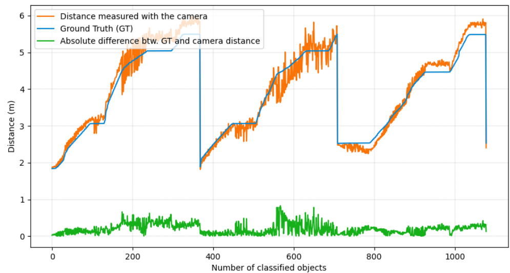
Figure 9. Measured distance between correctly classified objects and D435 RealSense camera (orange), ground truth distance (blue), absolute value of the difference between the ground truth distance and the distance estimated by the camera (green). The detected objects are sorted by class, then detection order.
