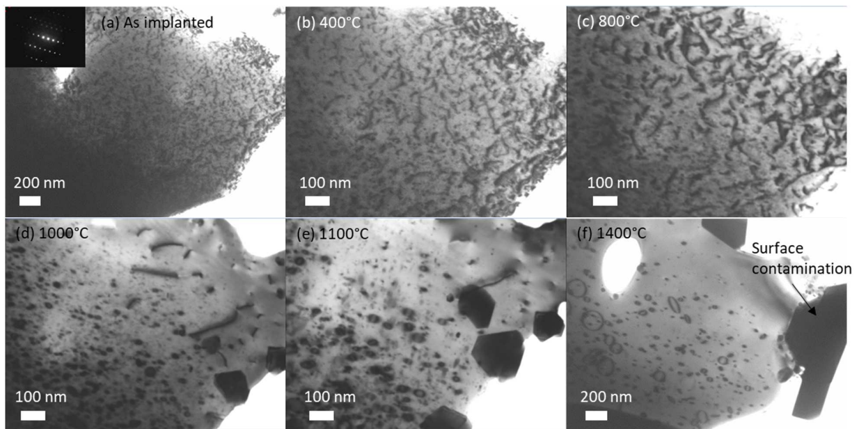
Figure 7 : Sequential BF TEM images of polycrystalline \text{UO}_2 thin foil irradiated with 4 MeV Au at 25 °C and 5 \times 10^{14} Au/cm 2 : (a) as implanted, (b) annealed at 400 °C, (c) 800 °C, (d) 1000 °C, (e) 1100 °C, (f) 1400 °C. The observations were carried out with g = 200 reflection. The inset shows the diffraction pattern.
