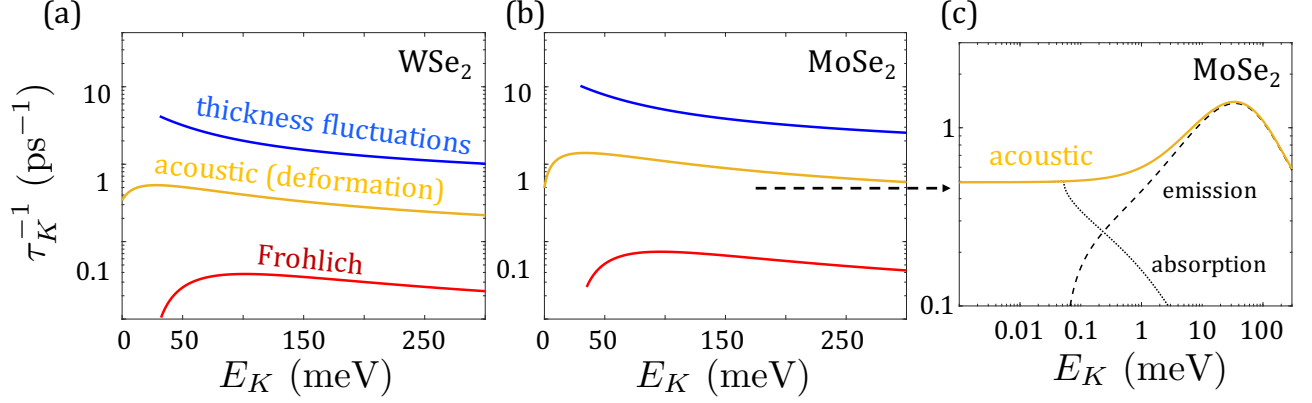
FIG. 5: Scattering rates in ML-WSe 2 (a) and ML-MoSe 2 (b) at T=5 K as a function of the exciton kinetic energy, E_K . (c) Breakup of the scattering rate into phonon emission and absorption components in the case of exciton interaction with acoustic phonons in ML-MoSe 2 .
