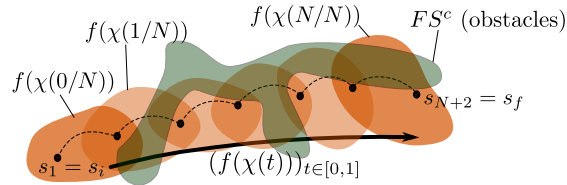
Fig. 4 From a valid continuous path (\chi(t))_{t \in [0,1]} \in \Omega^{[0,1]} to a valid finite sequence of configurations in CS.
