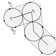
Fig. 1: Defining the markers for a particle in 2D
