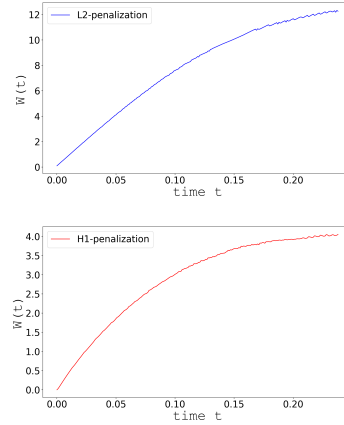
Fig. 3: W -component of the translational velocity reaching a terminal velocity for the L2-penalty (above) and H1-penalty (bottom)
