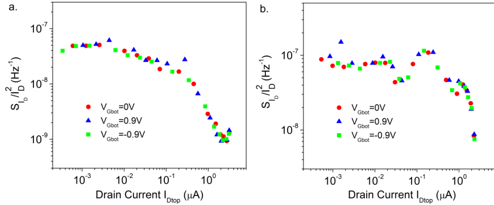
Fig. 6. Normalized power spectral density at f = 10\text{ Hz} vs drain current for a top NMOS with W = 2\mu\text{m} , L = 1\mu\text{m} (a) L = 0.1\mu\text{m} (b) and all bias cases of Table I.
