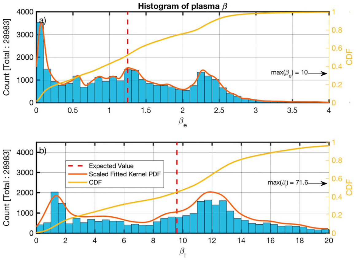
Figure 14. Histograms of the calculated plasma beta for the electrons (panel a) and ions (panel b) for the minimum variance analysis subintervals for which \omega_{rf} > \omega_{LH} . The estimated scaled fitted PDF and the CDF are also shown in red and yellow, respectively. The calculated average is shown by the dashed vertical red line. CDF = cumulative density function; PDF = probability density function.
