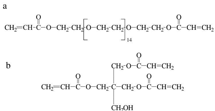
Fig. 1. a) Poly(ethylene glycol) diacrylate (PEGDA) and b) Pentaerythritoltriacylate (PETIA) monomers.
