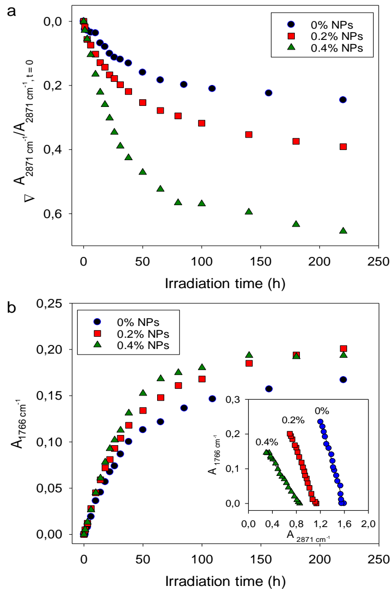
Fig. 11. Comparison of kinetic evolution of a) the decay of methylene groups (band at 2871 \text{ cm}^{-1} ) and b) the formation of ester groups (band at 1766 \text{ cm}^{-1} ) for the pure and Ag NPs dispersed PEGDA/PETIA polymer (0.2 and 0.4 % of NPs) upon irradiation. Inset: Correlation between the band at 2871 \text{ cm}^{-1} (CH 2 groups) and the band at 1766 \text{ cm}^{-1} (ester groups) of pure and doped polymer.
