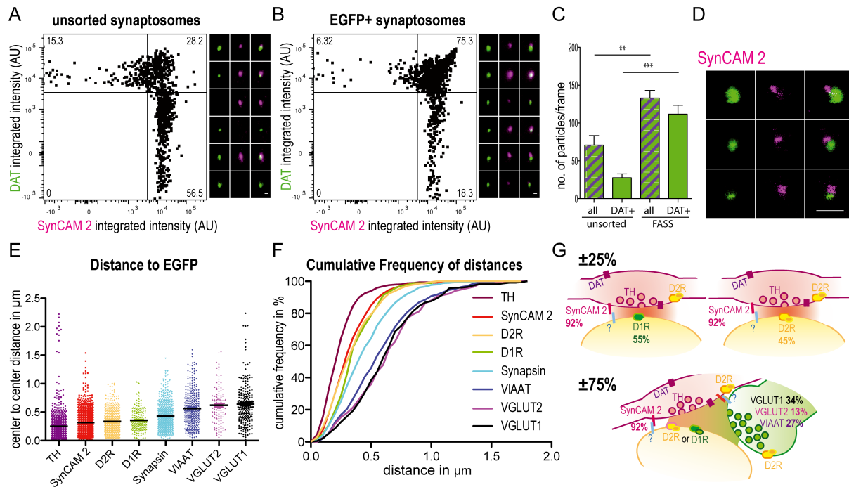
Figure 4: (A-B) Dot plots of anti-SynCAM 2 (x-axis) and anti-DAT (y-axis) intensity signals of unsorted and DAT-EGFP+ FASS synaptosomes (left). Representative epifluorescence images display a frequent tight apposition of SynCAM 2 and DAT. Note the strong enrichment of DAT+/SynCAM 2+ synaptosomes from 28.2% to 75.3% upon sorting (upper right quadrant). Instead, DAT-/SynCAM 2+ synaptosomes are 3-fold reduced as expected during sorting (lower right quadrant). (C) Quantification of (A) and (B) showing the number of particles per frame. n=3 sorts, mean \pm SEM. *** p < 0.001 , ** p < 0.01 . paired t-test. (D) STED images of synaptosomes stained for DAT (green) and SynCAM 2 (magenta). Scale bars 1 \mu m. (E) Distance to EGFP signal center of all stained proteins in increasing order of average distance. (F) Cumulative frequency distribution of distances to EGFP (percentage of all stained molecules). Note the proximity of SynCAM 2 to EGFP and the larger gap left by VGLUT and VIAAT varicosities. (G) Model of cellular and molecular architecture of dopamine synapses. Dopamine secretion sites labeled by the DAT-cre strategy are apposed to a postsynaptic element with either D1R (55%) or D2R (45%). In 92% of the cases SynCAM 2 seems to be involved in the synaptic architecture. Though SynCAM1 is a strong candidate,
