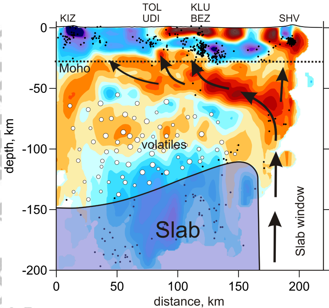
Figure 15. Schematic representation of feeding the volcanoes of NGV from the slab window. The background is the distribution of the S wave velocity anomalies in Section 1A-1B, same as in Figure 9. The black dots are the earthquake hypocenters. The white circles schematically indicate flow of volatiles from the slab; black arrows depict possible flow in the mantle wedge. The dotted line shows approximate location of the Moho interface.
