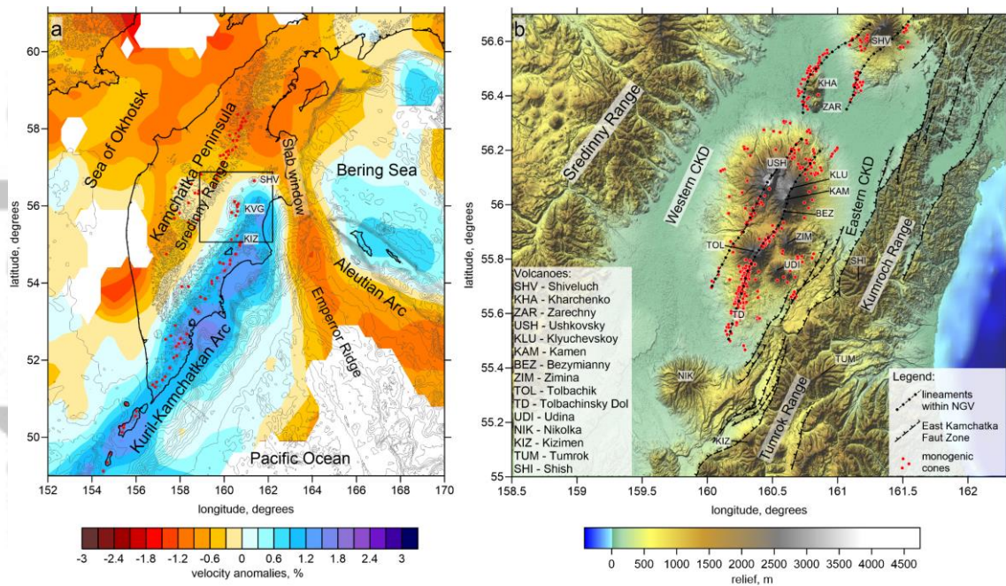
Figure 1. Geological framework of the study area. a. Major regional structures in the Kamchatka Peninsula and surrounding regions. Background is the horizontal section at 150 km depth of the P-wave velocity anomalies from the regional tomography model by Koulakov et al. (2011a). Thin contours indicate the topography/bathymetry variations with the interval of 500 m. Rectangle indicate the area shown in b. b. Major structural elements and volcanoes within the study area. Red dots are the monogenic cones from different sources (Volynets et al., 1998; Churikova et al. 2015) and authors' interpretation. Blue marks for volcanoes indicate their predominantly basaltic composition and yellow – silicic. The green mark for the Klyuchevskoy indicates the particular intermediate properties of this volcano. East Kamchatka Fault Zone is drawn based on (Kozhurin & Zelenin, 2017). Lineaments along the NGV are according to (Ermakov et al., 1973; Melekesetsev et al., 1991) and the author's own interpretation.
