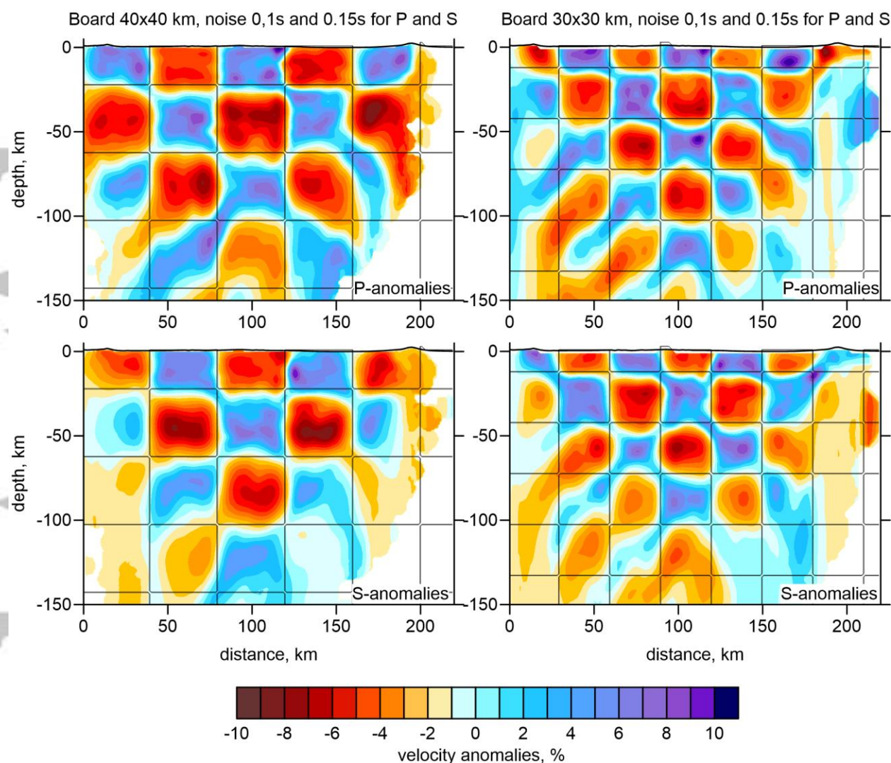
Figure 7. Checkerboard test for checking the vertical resolution for the P and S wave velocity anomalies. The synthetic anomalies are defined along the Section 1 (same as in Figure 11). The shapes of the synthetic anomalies are highlighted with black lines.
