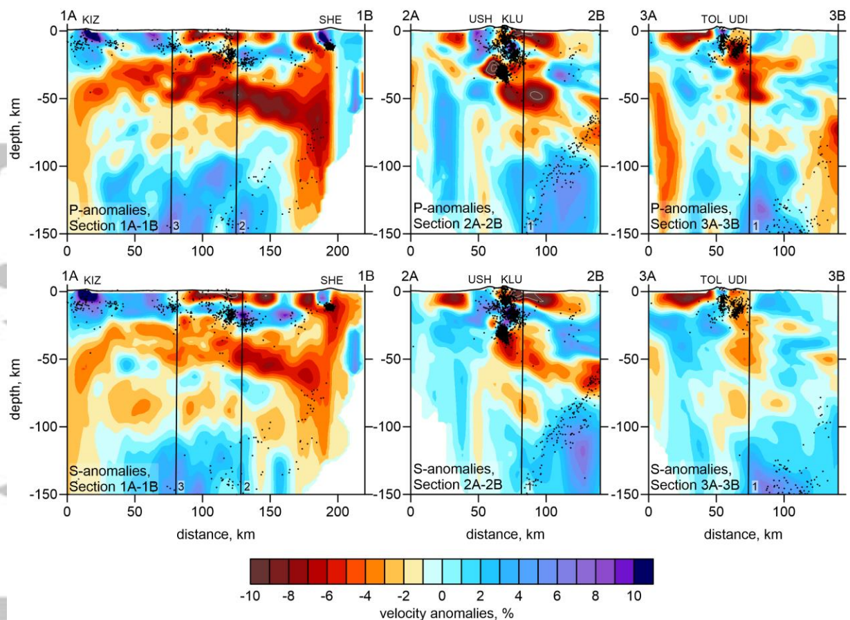
Figure 13. P and S wave velocity anomalies in three vertical sections indicated in Figure 10. Black dots indicate the seismicity along the profile (at distances less than 10 km). Names of the volcanoes are same as in Figure 1b. Vertical lines indicate intersections with other profiles.
