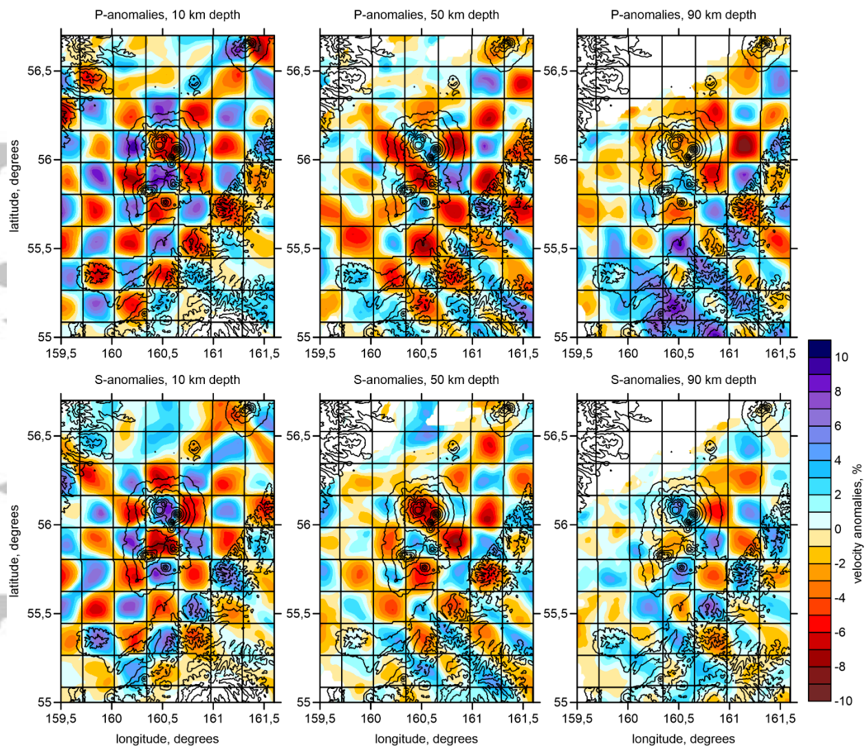
Figure 5. Checkerboard tests for the P and S wave velocity anomalies. Horizontal size of the anomalies in the synthetic model is 20x20 km. With depth, the sign of the anomalies changes at 30 km, 70 km, and 110 km. The shapes of the synthetic anomalies are shown with black lines. Contour lines indicate the topography with the interval of 500 m.
