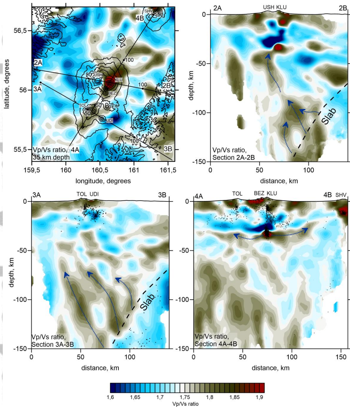
Figure 14. Vp/Vs ratio in one horizontal and three vertical sections. Blue dotted lines depict volatile flows, as discussed in the text. Contour lines in the map indicate the topography with the interval of 500 m. Names of the volcanoes are same as in Figure 1b. Dots in the vertical sections depict projections of events located at distances less than 10 km.
