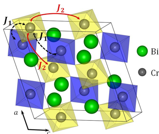
FIG. 3. Schematic representation of exchange paths in the unit cell of BCO (oxygen atoms placed at the octahedra vertices).
